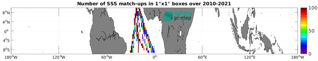
Figure 4: Number of SSS match-ups between TSG (Polarstern) SSS and the SMOS SSS L2Q v331 - No FLAG (CMEMS-CATDS-CPDC) SSS product for the Equatorial Ocean 10N-10S Pi-MEP region over 1^\circ \times 1^\circ boxes and for the full satellite product period.
