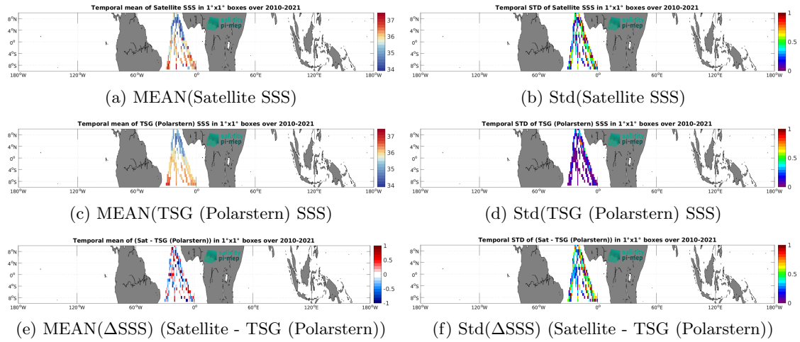
Figure 6: Temporal mean (left) and Std (right) of SSS from SMOS SSS L2Q v331 - No FLAG (CMEMS-CATDS-CPDC) (top), TSG (Polarstern) (middle), and of \Delta SSS (Satellite - TSG (Polarstern)). Only match-up pairs are used to generate these maps.
