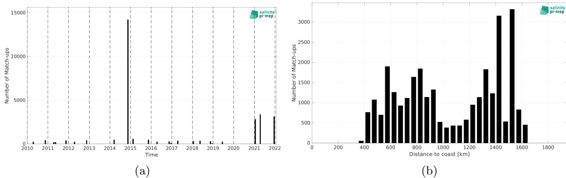
Figure 1: Number of match-ups between TSG (Polarstern) and SMOS SSS L2Q v331 - No FLAG (CMEMS-CATDS-CPDC) SSS as a function of time (a) and as function of the distance to coast (b) over the Equatorial Ocean 10N-10S Pi-MEP region and for the full satellite product period.
