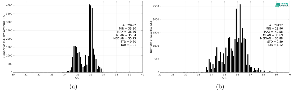
Figure 2: Histograms of SSS from TSG (Polarstern) (a) and SMOS SSS L2Q v331 - No FLAG (CMEMS-CATDS-CPDC) (b) considering all match-up pairs per bins of 0.1 over the Equatorial Ocean 10N-10S Pi-MEP region and for the full satellite product period.
