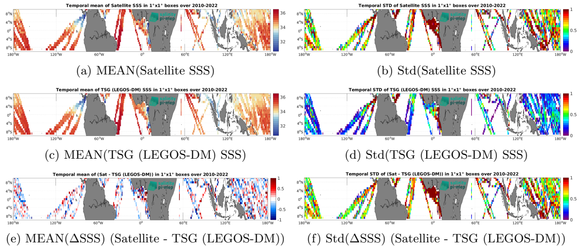
Figure 7: Temporal mean (left) and Std (right) of SSS from SMOS SSS L2Q v331 - No FLAG (CMEMS-CATDS-CPDC) (top), TSG (LEGOS-DM) (middle), and of \Delta SSS (Satellite - TSG (LEGOS-DM)). Only match-up pairs are used to generate these maps.
