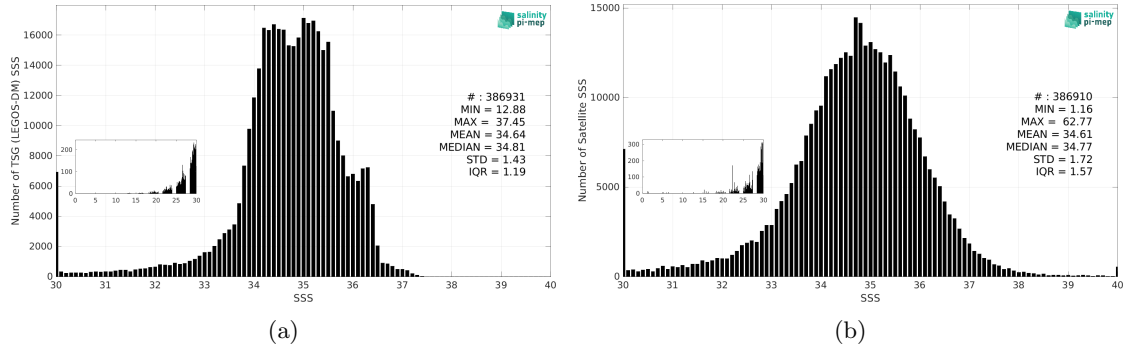
Figure 3: Histograms of SSS from TSG (LEGOS-DM) (a) and SMOS SSS L2Q v331 - No FLAG (CMEMS-CATDS-CPDC) (b) considering all match-up pairs per bins of 0.1 over the Equatorial Ocean 10N-10S Pi-MEP region and for the full satellite product period.
