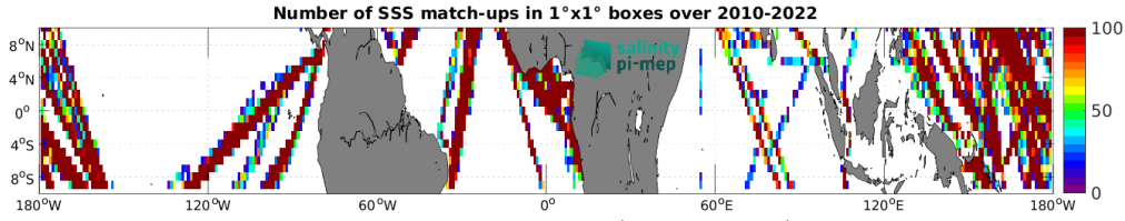
Figure 5: Number of SSS match-ups between TSG (LEGOS-DM) SSS and the SMOS SSS L2Q v331 - No FLAG (CMEMS-CATDS-CPDC) SSS product for the Equatorial Ocean 10N-10S Pi-MEP region over 1^\circ \times 1^\circ boxes and for the full satellite product period.
