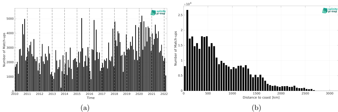
Figure 2: Number of match-ups between TSG (LEGOS-DM) and SMOS SSS L2Q v331 - No FLAG (CMEMS-CATDS-CPDC) SSS as a function of time (a) and as function of the distance to coast (b) over the Equatorial Ocean 10N-10S Pi-MEP region and for the full satellite product period.
