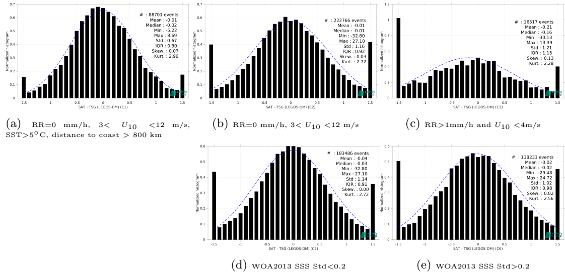
Figure 13: Normalized histogram of \Delta SSS (SMOS SSS L2Q v331 - No FLAG (CMEMS-CATDS-CPDC) - TSG (LEGOS-DM)) for 5 different subdatasets corresponding to: RR=0 mm/h, 3 < U_{10} < 12 m/s, SST >5^\circ C, distance to coast > 800 km (a), RR=0 mm/h, 3 < U_{10} < 12 m/s (b), RR >1 mm/h and U_{10} < 4 m/s (c), WOA2013 SSS Std <0.2 (d), WOA2013 SSS Std >0.2 (e).
