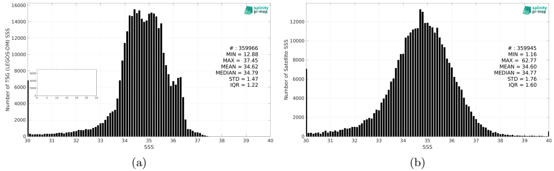
Figure 2: Histograms of SSS from TSG (LEGOS-DM) (a) and SMOS SSS L2Q v331 - No FLAG (CMEMS-CATDS-CPDC) (b) considering all match-up pairs per bins of 0.1 over the Equatorial Ocean 10N-10S Pi-MEP region and for the full satellite product period.
