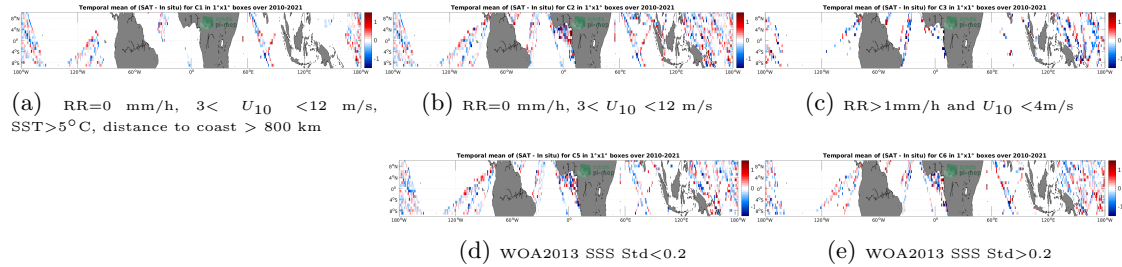
Figure 12: Temporal mean gridded over spatial boxes of size 1^{\circ}\times 1^{\circ} of \Delta\text{SSS} (SMOS SSS L2Q v331 - No FLAG (CMEMS-CATDS-CPDC) - TSG (LEGOS-DM)) for 5 different subdatasets corresponding to:RR=0 mm/h, 3 < U_{10} < 12 m/s, SST >5^{\circ}\text{C} , distance to coast > 800 km (a), RR=0 mm/h, 3 < U_{10} < 12 m/s (b), RR >1 mm/h and U_{10} < 4 m/s (c), WOA2013 SSS Std <0.2 (d), WOA2013 SSS Std >0.2 (e).
