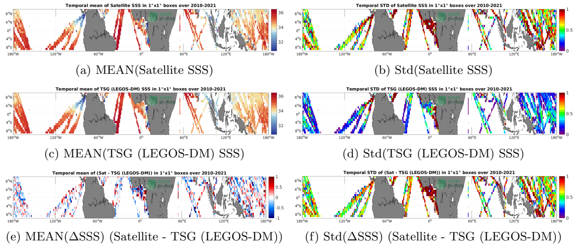
Figure 6: Temporal mean (left) and Std (right) of SSS from SMOS SSS L2Q v331 - No FLAG (CMEMS-CATDS-CPDC) (top), TSG (LEGOS-DM) (middle), and of \Delta SSS (Satellite - TSG (LEGOS-DM)). Only match-up pairs are used to generate these maps.
