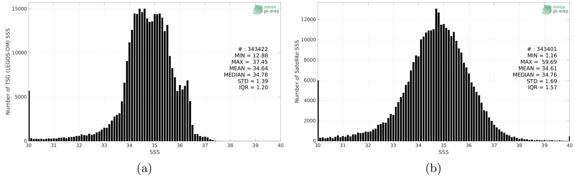
Figure 2: Histograms of SSS from TSG (LEGOS-DM) (a) and SMOS SSS L2Q v331 - No FLAG (CMEMS-CATDS-CPDC) (b) considering all match-up pairs per bins of 0.1 over the Equatorial Ocean 10N-10S Pi-MEP region and for the full satellite product period.
