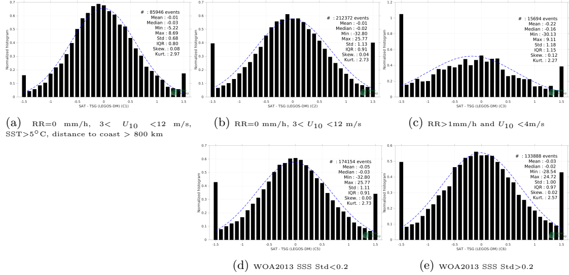
Figure 13: Normalized histogram of \Delta SSS (SMOS SSS L2Q v331 - No FLAG (CMEMS-CATDS-CPDC) - TSG (LEGOS-DM)) for 5 different subdatasets corresponding to: RR=0 mm/h, 3 < U_{10} < 12 m/s, SST>5°C, distance to coast > 800 km (a), RR=0 mm/h, 3 < U_{10} < 12 m/s (b), RR>1mm/h and U_{10} < 4 m/s (c), WOA2013 SSS Std<0.2 (d), WOA2013 SSS Std>0.2 (e).
