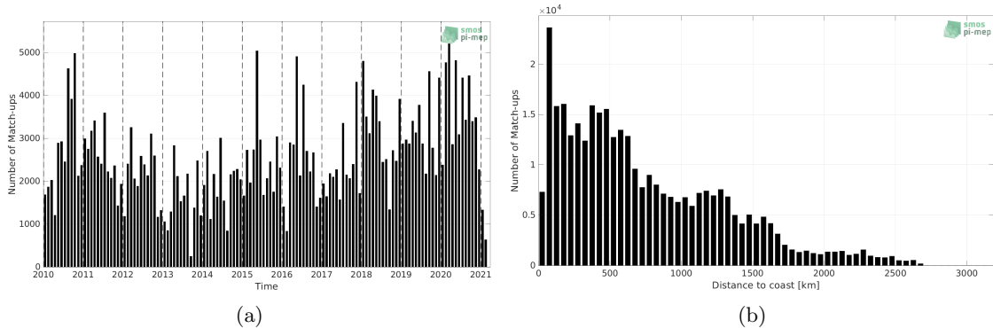
Figure 1: Number of match-ups between TSG (LEGOS-DM) and SMOS SSS L2Q v331 - No FLAG (CMEMS-CATDS-CPDC) SSS as a function of time (a) and as function of the distance to coast (b) over the Equatorial Ocean 10N-10S Pi-MEP region and for the full satellite product period.
