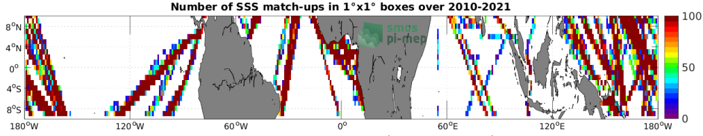
Figure 4: Number of SSS match-ups between TSG (LEGOS-DM) SSS and the SMOS SSS L2Q v331 - No FLAG (CMEMS-CATDS-CPDC) SSS product for the Equatorial Ocean 10N-10S Pi-MEP region over 1^\circ \times 1^\circ boxes and for the full satellite product period.
