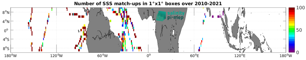
Figure 5: Number of SSS match-ups between TSG (GOSUD-Sailing-ship) SSS and the SMOS SSS L2Q v331 - No FLAG (CMEMS-CATDS-CPDC) SSS product for the Equatorial Ocean 10N-10S Pi-MEP region over 1^\circ \times 1^\circ boxes and for the full satellite product period.
