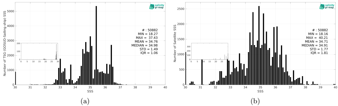
Figure 3: Histograms of SSS from TSG (GOSUD-Sailing-ship) (a) and SMOS SSS L2Q v331 - No FLAG (CMEMS-CATDS-CPDC) (b) considering all match-up pairs per bins of 0.1 over the Equatorial Ocean 10N-10S Pi-MEP region and for the full satellite product period.
