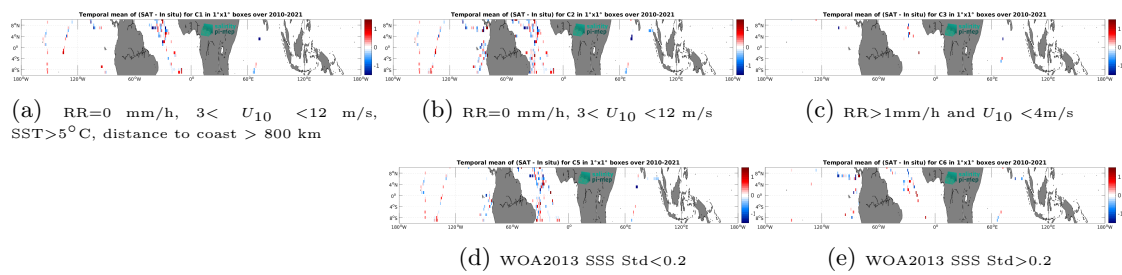
Figure 14: Temporal mean gridded over spatial boxes of size 1^\circ \times 1^\circ of \Delta\text{SSS} (SMOS SSS L2Q v331 - No FLAG (CMEMS-CATDS-CPDC) - TSG (GOSUD-Sailing-ship)) for 5 different sub-datasets corresponding to: RR=0 mm/h, 3 < U_{10} < 12 m/s, SST > 5°C, distance to coast > 800 km (a), RR=0 mm/h, 3 < U_{10} < 12 m/s (b), RR > 1mm/h and U_{10} < 4 m/s (c), WOA2013 SSS Std < 0.2 (d), WOA2013 SSS Std > 0.2 (e).
