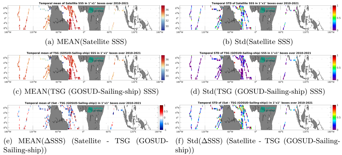
Figure 7: Temporal mean (left) and Std (right) of SSS from SMOS SSS L2Q v331 - No FLAG (CMEMS-CATDS-CPDC) (top), TSG (GOSUD-Sailing-ship) (middle), and of \Delta SSS (Satellite - TSG (GOSUD-Sailing-ship)). Only match-up pairs are used to generate these maps.
