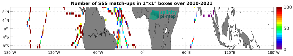
Figure 4: Number of SSS match-ups between TSG (GOSUD-Sailing-ship) SSS and the SMOS SSS L2Q v331 - No FLAG (CMEMS-CATDS-CPDC) SSS product for the Equatorial Ocean 10N-10S Pi-MEP region over 1^\circ \times 1^\circ boxes and for the full satellite product period.
