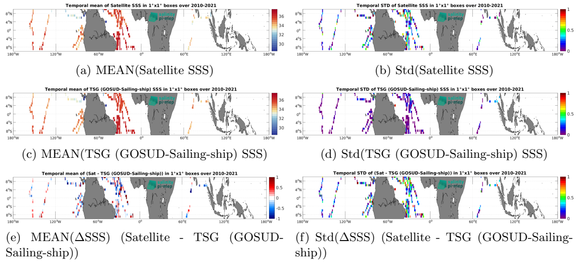
Figure 6: Temporal mean (left) and Std (right) of SSS from SMOS SSS L2Q v331 - No FLAG (CMEMS-CATDS-CPDC) (top), TSG (GOSUD-Sailing-ship) (middle), and of \Delta SSS (Satellite - TSG (GOSUD-Sailing-ship)). Only match-up pairs are used to generate these maps.
