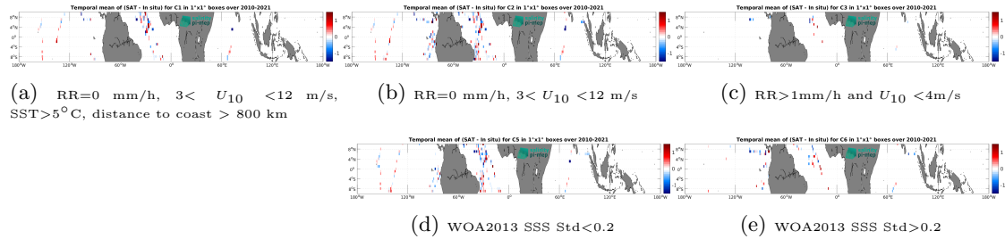
Figure 12: Temporal mean gridded over spatial boxes of size 1^{\circ}\times 1^{\circ} of \Delta SSS (SMOS SSS L2Q v331 - No FLAG (CMEMS-CATDS-CPDC) - TSG (GOSUD-Sailing-ship)) for 5 different sub-datasets corresponding to:RR=0 mm/h, 3 < U_{10} < 12 m/s, SST >5^{\circ}\text{C} , distance to coast > 800 km (a), RR=0 mm/h, 3 < U_{10} < 12 m/s (b), RR >1 mm/h and U_{10} < 4 m/s (c), WOA2013 SSS Std <0.2 (d), WOA2013 SSS Std >0.2 (e).
