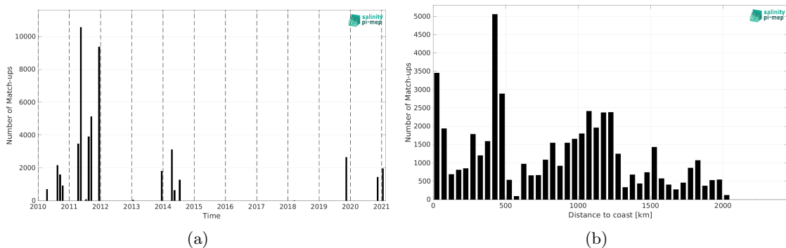
Figure 1: Number of match-ups between TSG (GOSUD-Sailing-ship) and SMOS SSS L2Q v331 - No FLAG (CMEMS-CATDS-CPDC) SSS as a function of time (a) and as function of the distance to coast (b) over the Equatorial Ocean 10N-10S Pi-MEP region and for the full satellite product period.
