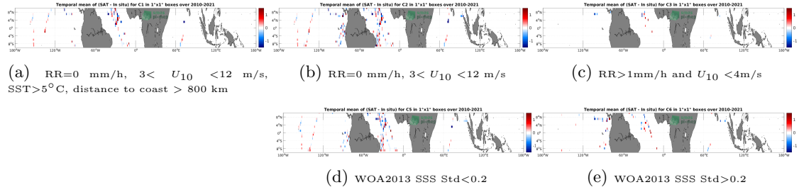
Figure 12: Temporal mean gridded over spatial boxes of size 1^{\circ}\times 1^{\circ} of \Delta SSS (SMOS SSS L2Q v331 - No FLAG (CMEMS-CATDS-CPDC) - TSG (GOSUD-Sailing-ship)) for 5 different sub-datasets corresponding to: RR=0 mm/h, 3 < U_{10} < 12 m/s, SST > 5^{\circ}\text{C} , distance to coast > 800 km (a), RR=0 mm/h, 3 < U_{10} < 12 m/s (b), RR > 1 mm/h and U_{10} < 4 m/s (c), WOA2013 SSS Std < 0.2 (d), WOA2013 SSS Std > 0.2 (e).
