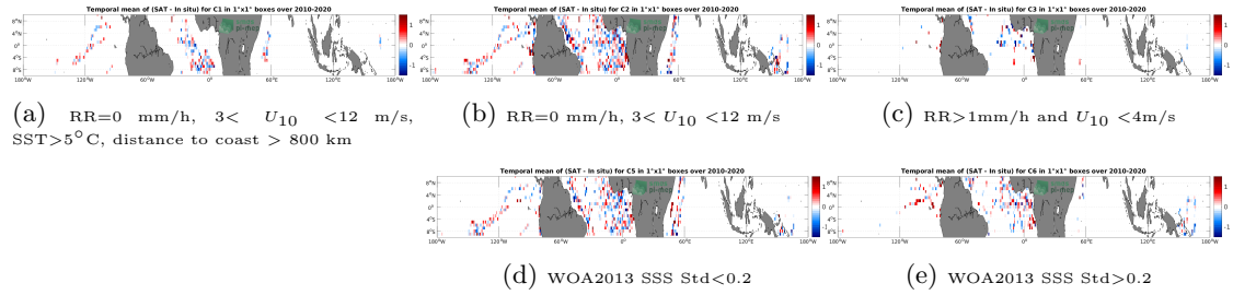
Figure 12: Temporal mean gridded over spatial boxes of size 1^{\circ}\times 1^{\circ} of \Delta SSS (SMOS SSS L2Q v331 - No FLAG (CMEMS-CATDS-CPDC) - TSG (GOSUD-Research-vessel)) for 5 different subdatasets corresponding to:RR=0 mm/h, 3 < U_{10} < 12 m/s, SST > 5^{\circ}\text{C} , distance to coast > 800 km (a), RR=0 mm/h, 3 < U_{10} < 12 m/s (b), RR > 1 mm/h and U_{10} < 4 m/s (c), WOA2013 SSS Std < 0.2 (d), WOA2013 SSS Std > 0.2 (e).
