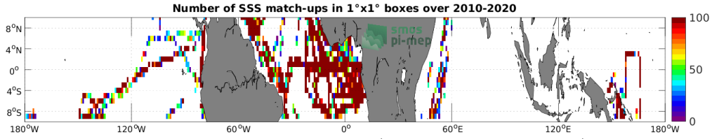
Figure 4: Number of SSS match-ups between TSG (GOSUD-Research-vessel) SSS and the SMOS SSS L2Q v331 - No FLAG (CMEMS-CATDS-CPDC) SSS product for the Equatorial Ocean 10N-10S Pi-MEP region over 1^\circ \times 1^\circ boxes and for the full satellite product period.
