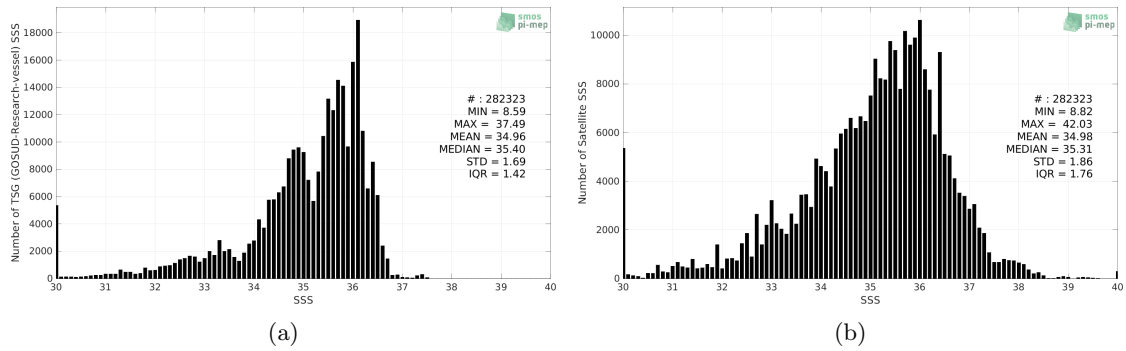
Figure 2: Histograms of SSS from TSG (GOSUD-Research-vessel) (a) and SMOS SSS L2Q v331 - No FLAG (CMEMS-CATDS-CPDC) (b) considering all match-up pairs per bins of 0.1 over the Equatorial Ocean 10N-10S Pi-MEP region and for the full satellite product period.
