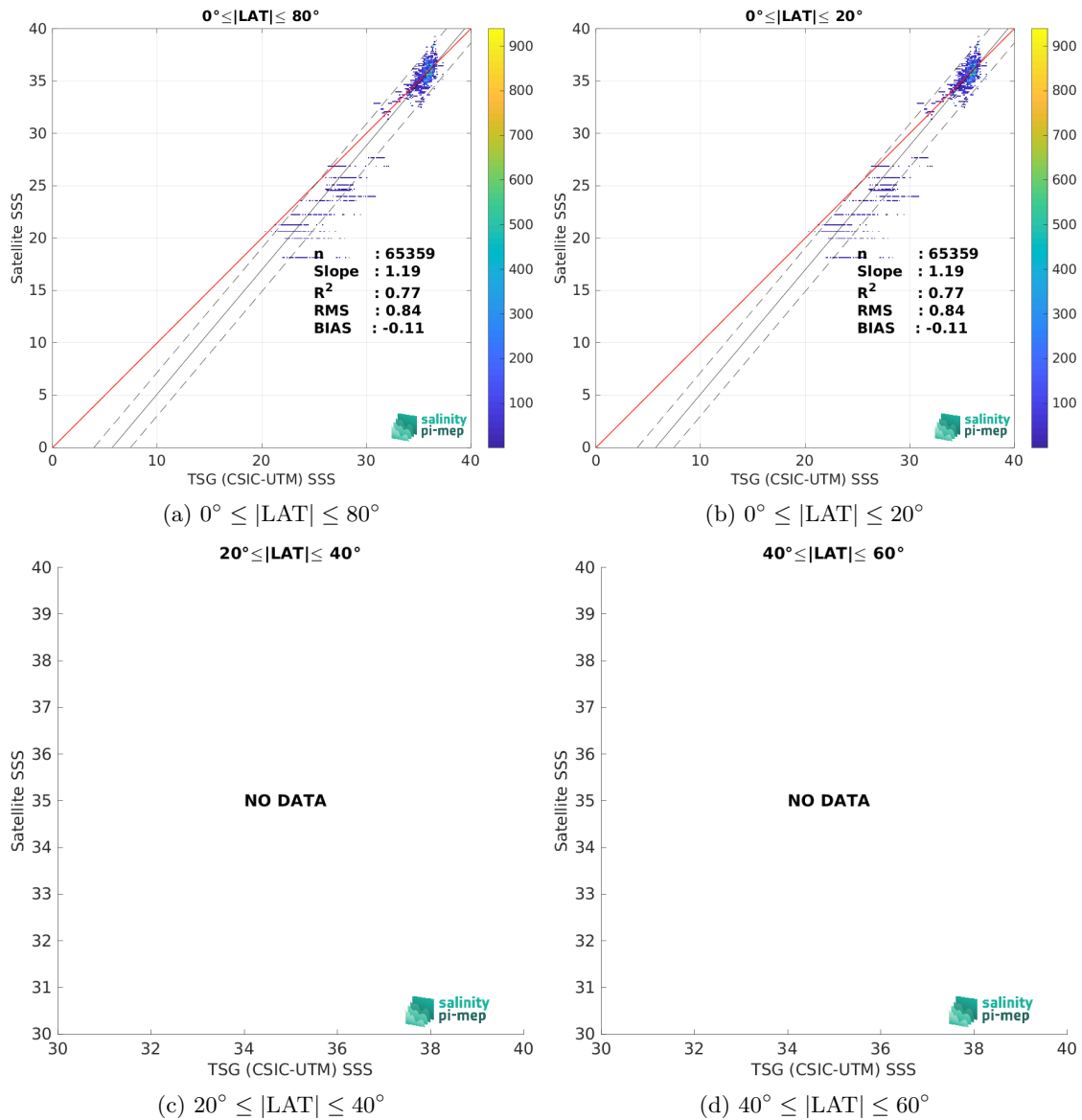
Figure 9: Contour maps of the concentration of SMOS SSS L2Q v331 - No FLAG (CMEMS-CATDS-CPDC) SSS ( y -axis) versus TSG (CSIC-UTM) SSS ( x -axis) at match-up pairs for different latitude bands. For each plot, the red line shows x=y . The black thin and dashed lines indicate a linear fit through the data cloud and the \pm 95\% confidence levels, respectively. The number match-up pairs n , the slope and R^2 coefficient of the linear fit, the root mean square (RMS) and the mean bias between satellite and in situ data are indicated for each latitude band in each plots.
