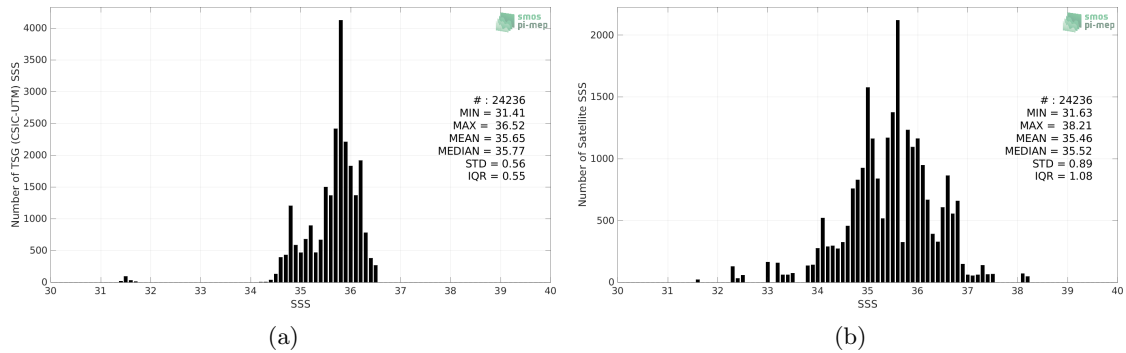
Figure 2: Histograms of SSS from TSG (CSIC-UTM) (a) and SMOS SSS L2Q v331 - No FLAG (CMEMS-CATDS-CPDC) (b) considering all match-up pairs per bins of 0.1 over the Equatorial Ocean 10N-10S Pi-MEP region and for the full satellite product period.
