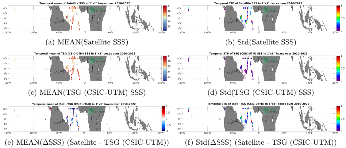
Figure 6: Temporal mean (left) and Std (right) of SSS from SMOS SSS L2Q v331 - No FLAG (CMEMS-CATDS-CPDC) (top), TSG (CSIC-UTM) (middle), and of \Delta SSS (Satellite - TSG (CSIC-UTM)). Only match-up pairs are used to generate these maps.
