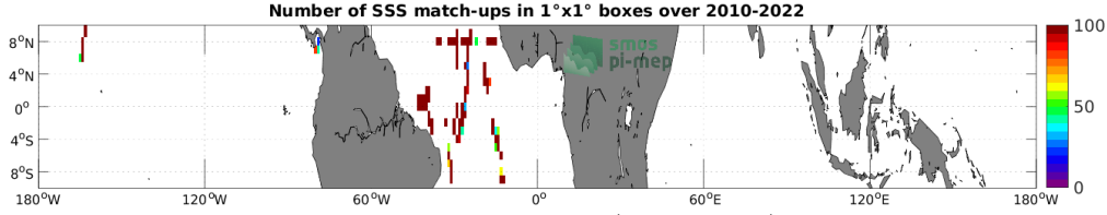
Figure 4: Number of SSS match-ups between TSG (CSIC-UTM) SSS and the SMOS SSS L2Q v331 - No FLAG (CMEMS-CATDS-CPDC) SSS product for the Equatorial Ocean 10N-10S Pi-MEP region over 1^\circ \times 1^\circ boxes and for the full satellite product period.
