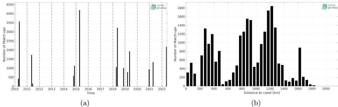
Figure 1: Number of match-ups between TSG (CSIC-UTM) and SMOS SSS L2Q v331 - No FLAG (CMEMS-CATDS-CPDC) SSS as a function of time (a) and as function of the distance to coast (b) over the Equatorial Ocean 10N-10S Pi-MEP region and for the full satellite product period.
