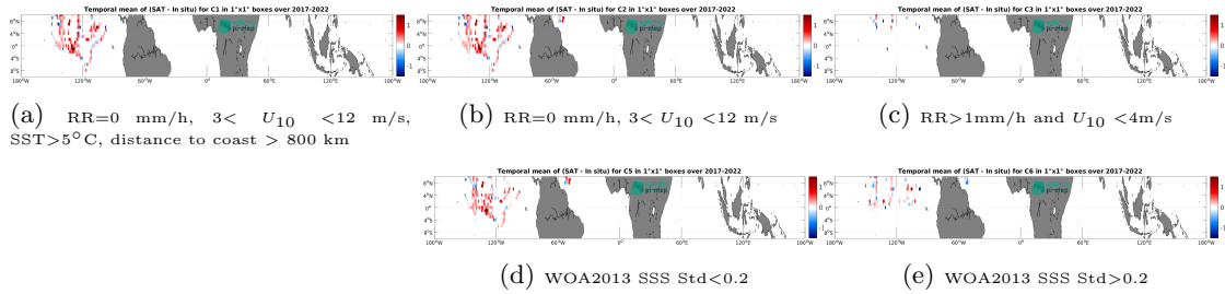
Figure 14: Temporal mean gridded over spatial boxes of size 1^\circ \times 1^\circ of \Delta\text{SSS} (SMOS SSS L2Q v331 - No FLAG (CMEMS-CATDS-CPDC) - Sailydrone) for 5 different subdatasets corresponding to: RR=0 mm/h, 3 < U_{10} < 12 m/s, SST>5°C, distance to coast > 800 km (a), RR=0 mm/h, 3 < U_{10} < 12 m/s (b), RR>1mm/h and U_{10} < 4 m/s (c), WOA2013 SSS Std<0.2 (d), WOA2013 SSS Std>0.2 (e).
