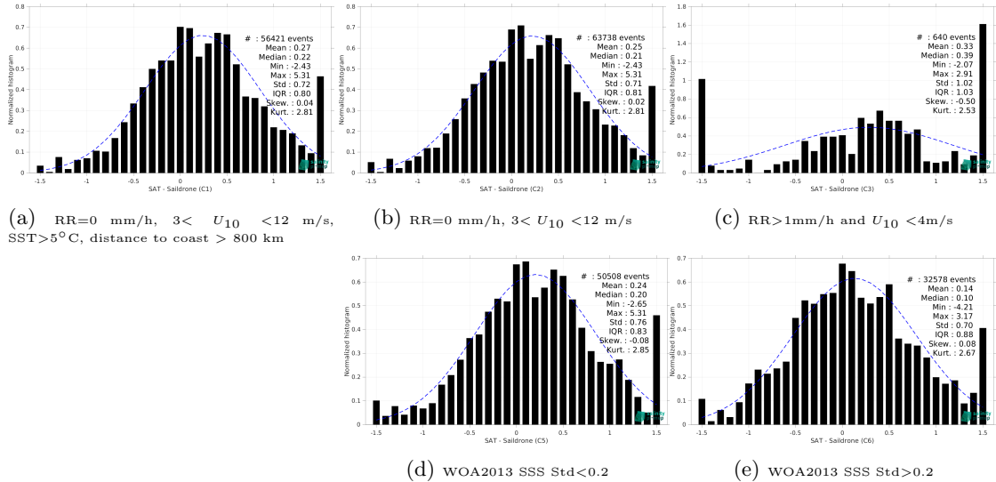
Figure 15: Normalized histogram of \Delta\text{SSS} (SMOS SSS L2Q v331 - No FLAG (CMEMS-CATDS-CPDC) - Sailydrone) for 5 different subdatasets corresponding to: RR=0 mm/h, 3 < U_{10} < 12 m/s, SST>5°C, distance to coast > 800 km (a), RR=0 mm/h, 3 < U_{10} < 12 m/s (b), RR>1mm/h and U_{10} < 4 m/s (c), WOA2013 SSS Std<0.2 (d), WOA2013 SSS Std>0.2 (e).
