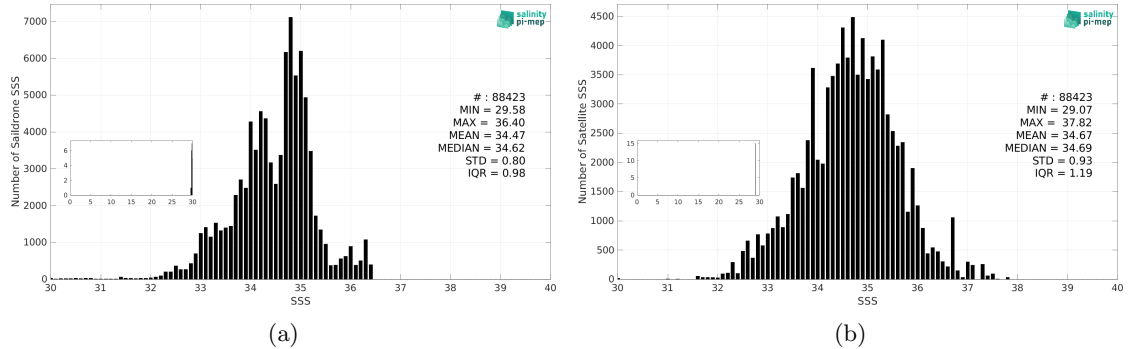
Figure 3: Histograms of SSS from Saildrone (a) and SMOS SSS L2Q v331 - No FLAG (CMEMS-CATDS-CPDC) (b) considering all match-up pairs per bins of 0.1 over the Equatorial Ocean 10N-10S Pi-MEP region and for the full satellite product period.
