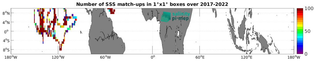
Figure 5: Number of SSS match-ups between Saildrone SSS and the SMOS SSS L2Q v331 - No FLAG (CMEMS-CATDS-CPDC) SSS product for the Equatorial Ocean 10N-10S Pi-MEP region over 1^\circ \times 1^\circ boxes and for the full satellite product period.
