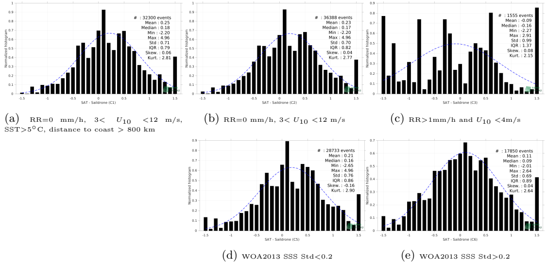
Figure 13: Normalized histogram of \Delta SSS (SMOS SSS L2Q v331 - No FLAG (CMEMS-CATDS-CPDC) - Saildrone) for 5 different subdatasets corresponding to: RR=0 mm/h, 3 < U_{10} < 12 m/s, SST >5^\circ C, distance to coast > 800 km (a), RR=0 mm/h, 3 < U_{10} < 12 m/s (b), RR >1 mm/h and U_{10} < 4 m/s (c), WOA2013 SSS Std <0.2 (d), WOA2013 SSS Std >0.2 (e).
