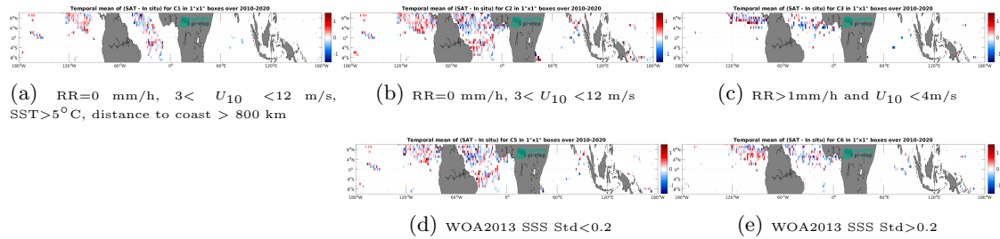
Figure 11: Temporal mean gridded over spatial boxes of size 1^\circ \times 1^\circ of \Delta SSS (SMOS SSS L2Q v331 - No FLAG (CMEMS-CATDS-CPDC) - Surface drifters) for 5 different subdatasets corresponding to:RR=0 mm/h, 3 < U_{10} < 12 m/s, SST >5^\circ C, distance to coast > 800 km (a), RR=0 mm/h, 3 < U_{10} < 12 m/s (b), RR >1 mm/h and U_{10} < 4 m/s (c), WOA2013 SSS Std <0.2 (d), WOA2013 SSS Std >0.2 (e).
