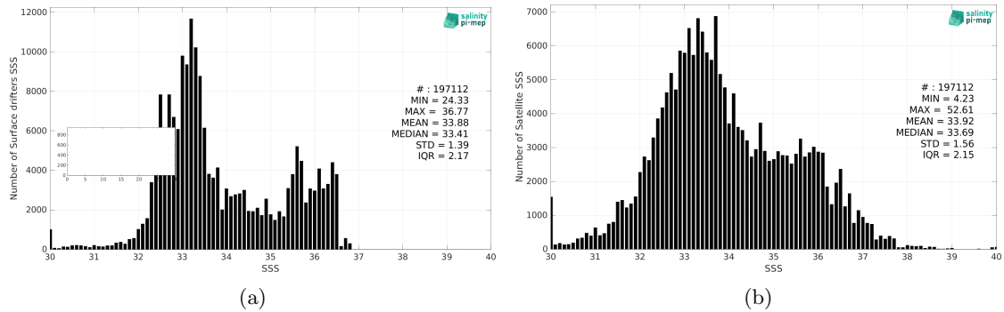
Figure 2: Histograms of SSS from Surface drifters (a) and SMOS SSS L2Q v331 - No FLAG (CMEMS-CATDS-CPDC) (b) considering all match-up pairs per bins of 0.1 over the Equatorial Ocean 10N-10S Pi-MEP region and for the full satellite product period.
