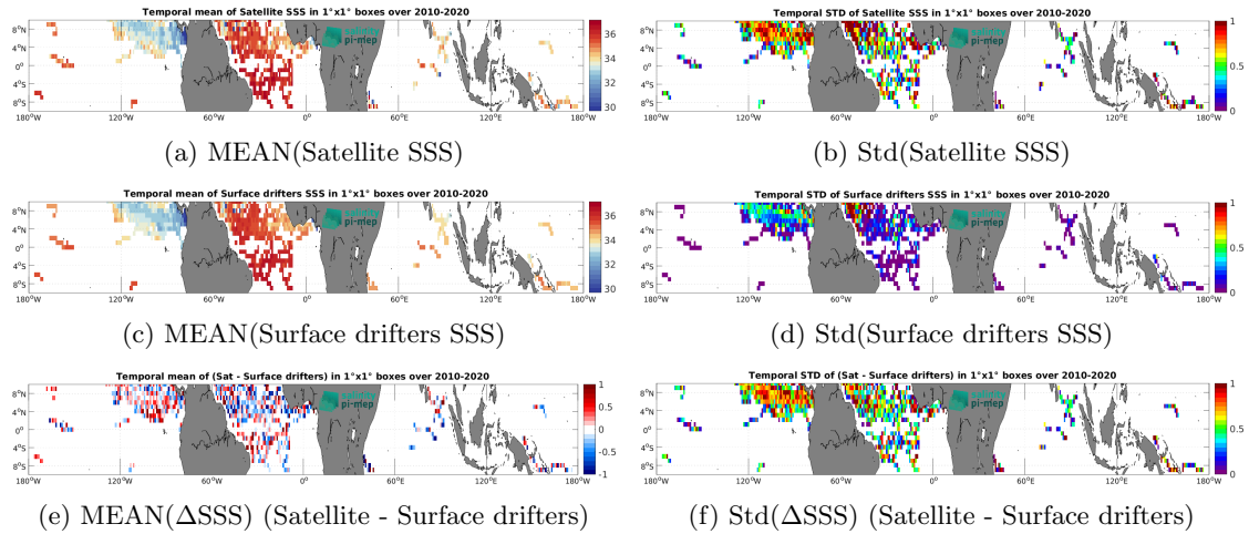
Figure 5: Temporal mean (left) and Std (right) of SSS from SMOS SSS L2Q v331 - No FLAG (CMEMS-CATDS-CPDC) (top), Surface drifters (middle), and of \Delta SSS (Satellite - Surface drifters). Only match-up pairs are used to generate these maps.
