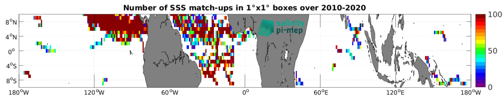
Figure 3: Number of SSS match-ups between Surface drifters SSS and the SMOS SSS L2Q v331 - No FLAG (CMEMS-CATDS-CPDC) SSS product for the Equatorial Ocean 10N-10S Pi-MEP region over 1^\circ \times 1^\circ boxes and for the full satellite product period.
