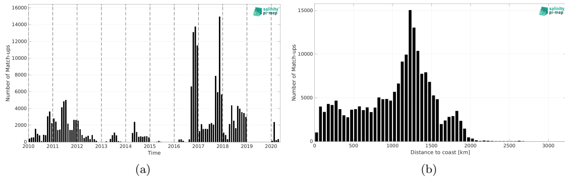
Figure 1: Number of match-ups between Surface drifters and SMOS SSS L2Q v331 - No FLAG (CMEMS-CATDS-CPDC) SSS as a function of time (a) and as function of the distance to coast (b) over the Equatorial Ocean 10N-10S Pi-MEP region and for the full satellite product period.
