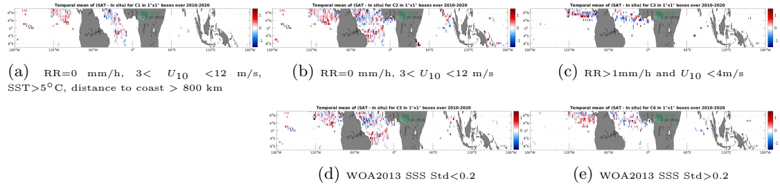
Figure 11: Temporal mean gridded over spatial boxes of size 1^{\circ}\times 1^{\circ} of \Delta\text{SSS} (SMOS SSS L2Q v331 - No FLAG (CMEMS-CATDS-CPDC) - Surface drifters) for 5 different subdatasets corresponding to:RR=0 mm/h, 3 < U_{10} < 12 m/s, SST >5^{\circ}\text{C} , distance to coast > 800 km (a), RR=0 mm/h, 3 < U_{10} < 12 m/s (b), RR >1 mm/h and U_{10} < 4 m/s (c), WOA2013 SSS Std <0.2 (d), WOA2013 SSS Std >0.2 (e).
