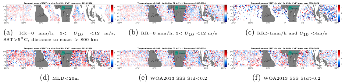
Figure 14: Temporal mean gridded over spatial boxes of size 1^\circ \times 1^\circ of \Delta\text{SSS} (SMOS SSS L2Q v331 - No FLAG (CMEMS-CATDS-CPDC) - Argo) for 6 different subdatasets corresponding to:RR=0 mm/h, 3 < U_{10} < 12 m/s, SST>5°C, distance to coast > 800 km (a), RR=0 mm/h, 3 < U_{10} < 12 m/s (b), RR>1mm/h and U_{10} < 4 m/s (c),MLD<20m (d),WOA2013 SSS Std<0.2 (e),WOA2013 SSS Std>0.2 (f).
