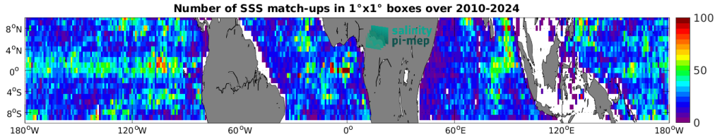
Figure 5: Number of SSS match-ups between Argo SSS and the SMOS SSS L2Q v331 - No FLAG (CMEMS-CATDS-CPDC) SSS product for the Equatorial Ocean 10N-10S Pi-MEP region over 1^\circ \times 1^\circ boxes and for the full satellite product period.
