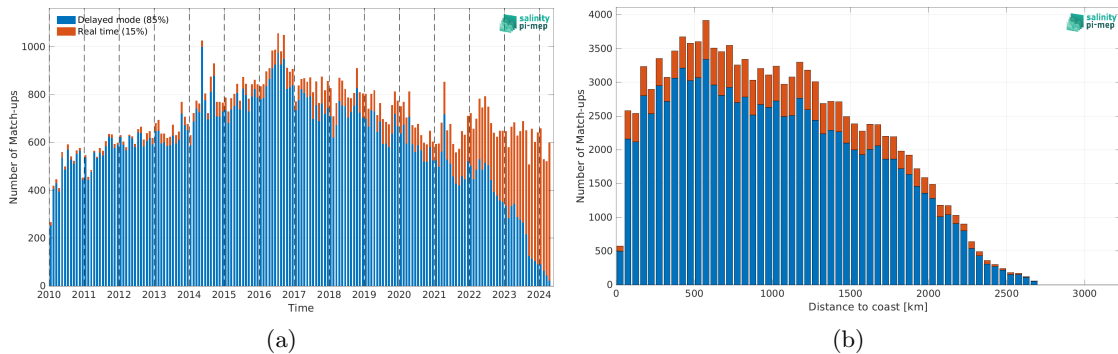
Figure 2: Number of match-ups between Argo and SMOS SSS L2Q v331 - No FLAG (CMEMS-CATDS-CPDC) SSS as a function of time (a) and as function of the distance to coast (b) over the Equatorial Ocean 10N-10S Pi-MEP region and for the full satellite product period.
