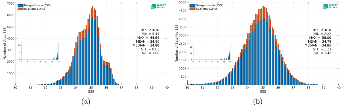
Figure 3: Histograms of SSS from Argo (a) and SMOS SSS L2Q v331 - No FLAG (CMEMS-CATDS-CPDC) (b) considering all match-up pairs per bins of 0.1 over the Equatorial Ocean 10N-10S Pi-MEP region and for the full satellite product period.
