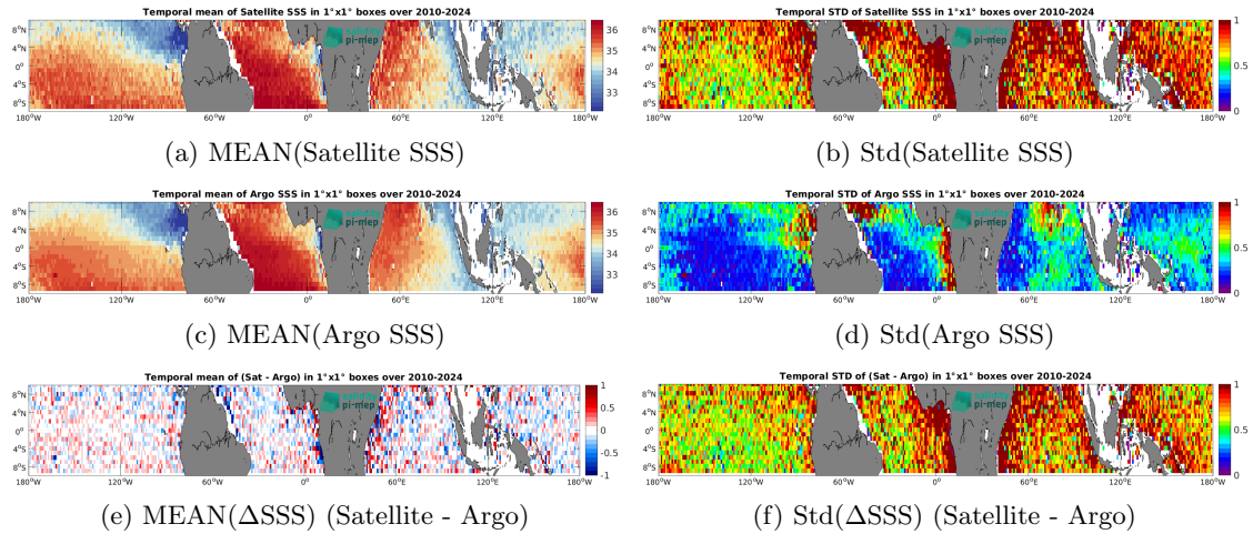
Figure 7: Temporal mean (left) and Std (right) of SSS from SMOS SSS L2Q v331 - No FLAG (CMEMS-CATDS-CPDC) (top), Argo (middle), and of \Delta SSS (Satellite - Argo). Only match-up pairs are used to generate these maps.
