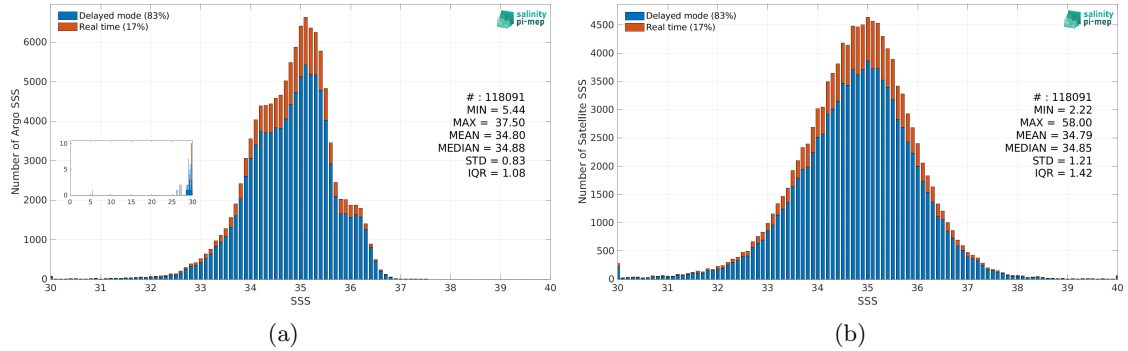
Figure 2: Histograms of SSS from Argo (a) and SMOS SSS L2Q v331 - No FLAG (CMEMS-CATDS-CPDC) (b) considering all match-up pairs per bins of 0.1 over the Equatorial Ocean 10N-10S Pi-MEP region and for the full satellite product period.
