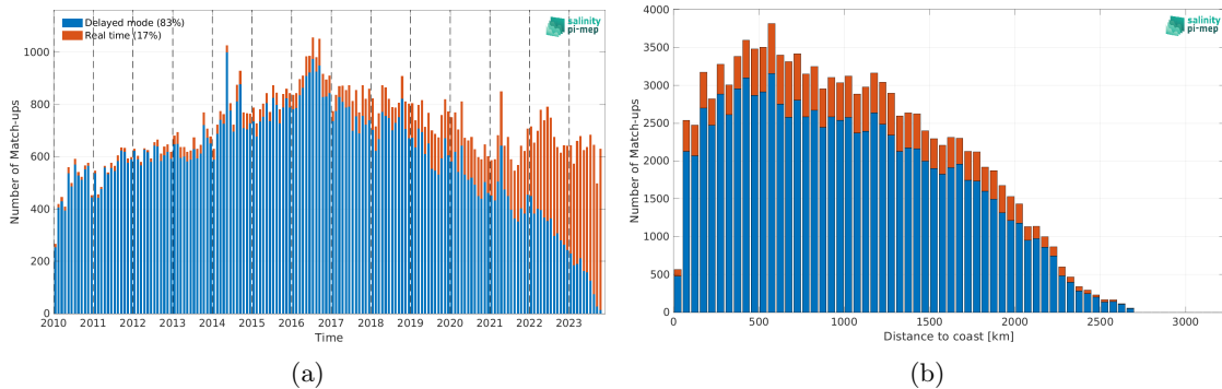
Figure 1: Number of match-ups between Argo and SMOS SSS L2Q v331 - No FLAG (CMEMS-CATDS-CPDC) SSS as a function of time (a) and as function of the distance to coast (b) over the Equatorial Ocean 10N-10S Pi-MEP region and for the full satellite product period.
