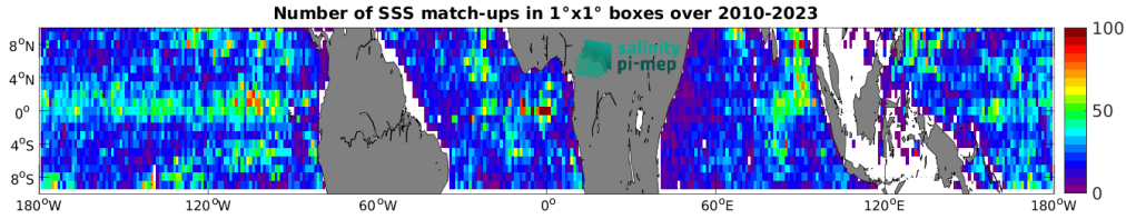
Figure 4: Number of SSS match-ups between Argo SSS and the SMOS SSS L2Q v331 - No FLAG (CMEMS-CATDS-CPDC) SSS product for the Equatorial Ocean 10N-10S Pi-MEP region over 1^\circ \times 1^\circ boxes and for the full satellite product period.
