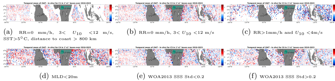
Figure 12: Temporal mean gridded over spatial boxes of size 1^\circ \times 1^\circ of \Delta SSS (SMOS SSS L2Q v331 - No FLAG (CMEMS-CATDS-CPDC) - Argo) for 6 different subdatasets corresponding to:RR=0 mm/h, 3 < U_{10} < 12 m/s, SST >5^\circ C, distance to coast > 800 km (a), RR=0 mm/h, 3 < U_{10} < 12 m/s (b), RR >1 mm/h and U_{10} < 4 m/s (c),MLD <20 m (d),WOA2013 SSS Std <0.2 (e),WOA2013 SSS Std >0.2 (f).
