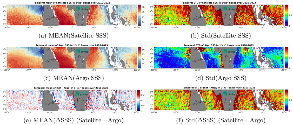
Figure 6: Temporal mean (left) and Std (right) of SSS from SMOS SSS L2Q v331 - No FLAG (CMEMS-CATDS-CPDC) (top), Argo (middle), and of \Delta SSS (Satellite - Argo). Only match-up pairs are used to generate these maps.
