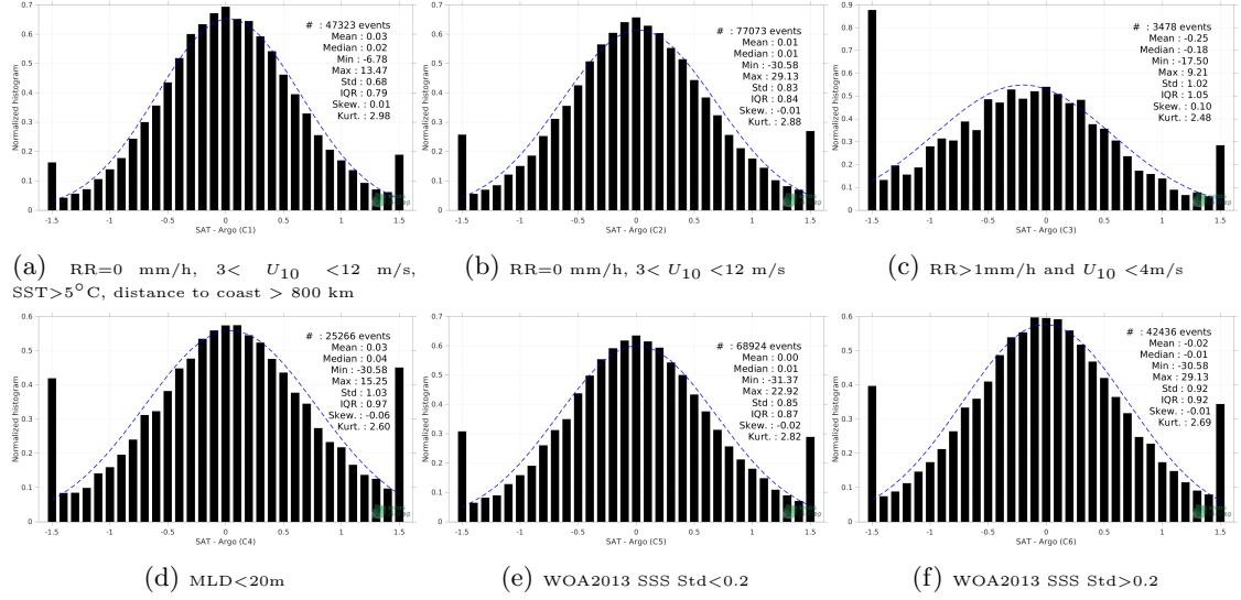
Figure 13: Normalized histogram of \Delta SSS (SMOS SSS L2Q v331 - No FLAG (CMEMS-CATDS-CPDC) - Argo) for 6 different subdatasets corresponding to: RR=0 mm/h, 3 < U_{10} < 12 m/s, SST > 5°C, distance to coast > 800 km (a), RR=0 mm/h, 3 < U_{10} < 12 m/s (b), RR > 1mm/h and U_{10} < 4 m/s (c), MLD < 20m (d), WOA2013 SSS Std < 0.2 (e), WOA2013 SSS Std > 0.2 (f).
