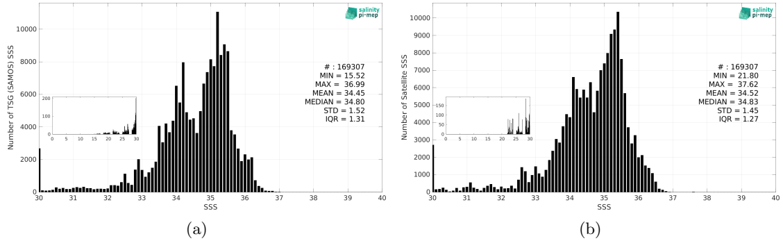
Figure 3: Histograms of SSS from TSG (SAMOS) (a) and SMOS SSS L3 v9 - 9 Days (CATDS-CEC-LOCEAN) (b) considering all match-up pairs per bins of 0.1 over the Equatorial Ocean 10N-10S Pi-MEP region and for the full satellite product period.
