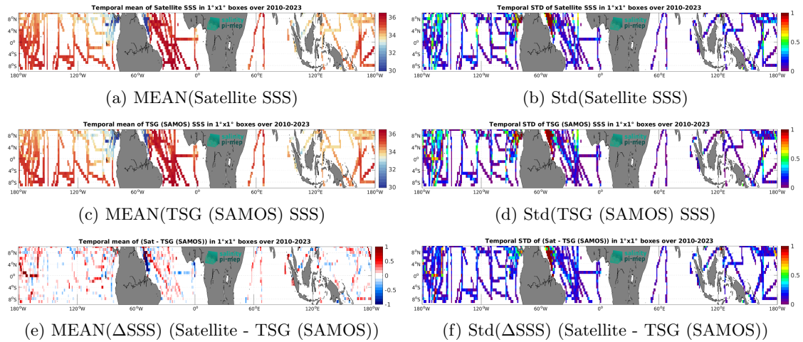
Figure 7: Temporal mean (left) and Std (right) of SSS from SMOS SSS L3 v9 - 9 Days (CATDS-CEC-LOCEAN) (top), TSG (SAMOS) (middle), and of \Delta SSS (Satellite - TSG (SAMOS)). Only match-up pairs are used to generate these maps.
