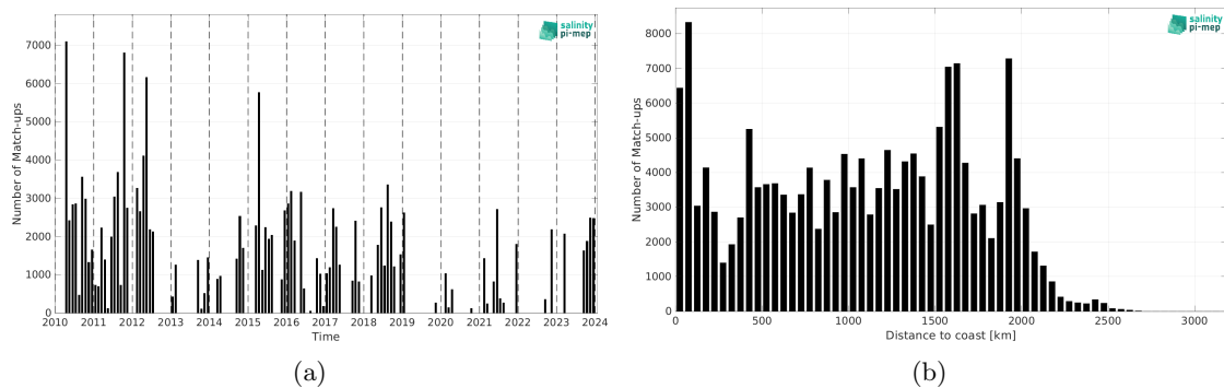
Figure 2: Number of match-ups between TSG (SAMOS) and SMOS SSS L3 v9 - 9 Days (CATDS-CEC-LOCEAN) SSS as a function of time (a) and as function of the distance to coast (b) over the Equatorial Ocean 10N-10S Pi-MEP region and for the full satellite product period.
