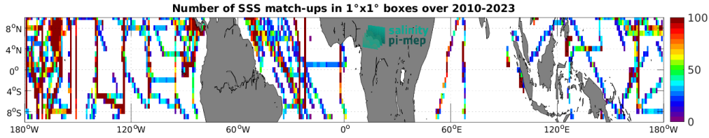
Figure 5: Number of SSS match-ups between TSG (SAMOS) SSS and the SMOS SSS L3 v9 - 9 Days (CATDS-CEC-LOCEAN) SSS product for the Equatorial Ocean 10N-10S Pi-MEP region over 1^\circ \times 1^\circ boxes and for the full satellite product period.
