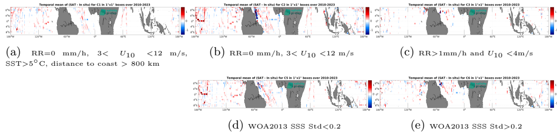
Figure 12: Temporal mean gridded over spatial boxes of size 1^\circ \times 1^\circ of \Delta SSS (SMOS SSS L3 v9 - 9 Days (CATDS-CEC-LOCEAN) - TSG (SAMOS)) for 5 different subdatasets corresponding to: RR=0 mm/h, 3 < U_{10} < 12 m/s, SST >5^\circ C, distance to coast > 800 km (a), RR=0 mm/h, 3 < U_{10} < 12 m/s (b), RR >1 mm/h and U_{10} < 4 m/s (c), WOA2013 SSS Std <0.2 (d), WOA2013 SSS Std >0.2 (e).
