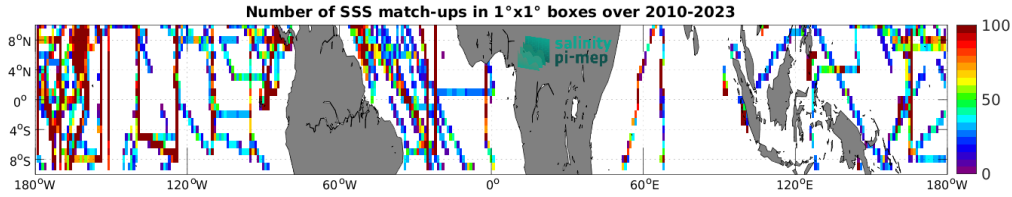
Figure 4: Number of SSS match-ups between TSG (SAMOS) SSS and the SMOS SSS L3 v9 - 9 Days (CATDS-CEC-LOCEAN) SSS product for the Equatorial Ocean 10N-10S Pi-MEP region over 1^\circ \times 1^\circ boxes and for the full satellite product period.
