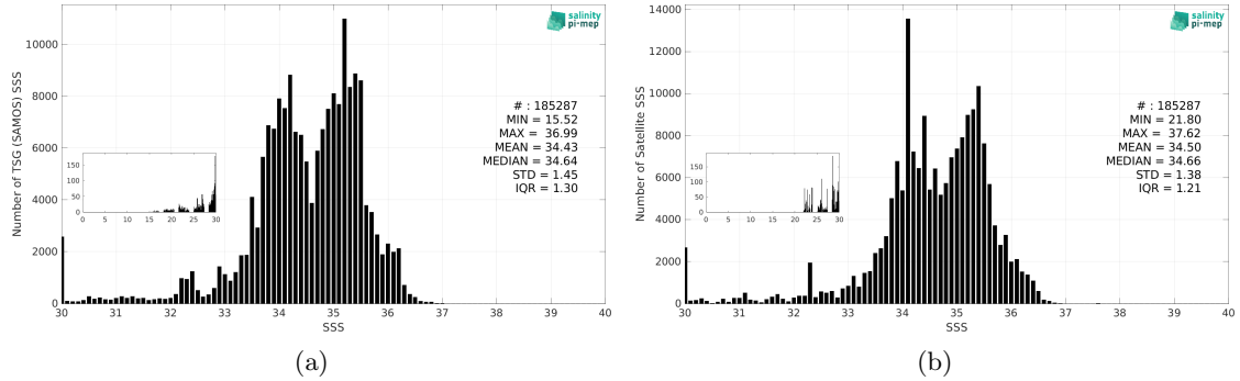
Figure 2: Histograms of SSS from TSG (SAMOS) (a) and SMOS SSS L3 v9 - 9 Days (CATDS-CEC-LOCEAN) (b) considering all match-up pairs per bins of 0.1 over the Equatorial Ocean 10N-10S Pi-MEP region and for the full satellite product period.
