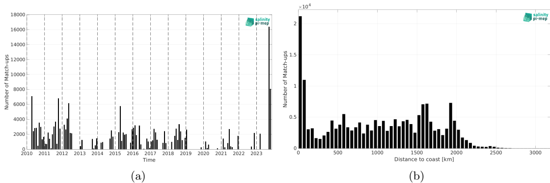
Figure 1: Number of match-ups between TSG (SAMOS) and SMOS SSS L3 v9 - 9 Days (CATDS-CEC-LOCEAN) SSS as a function of time (a) and as function of the distance to coast (b) over the Equatorial Ocean 10N-10S Pi-MEP region and for the full satellite product period.
