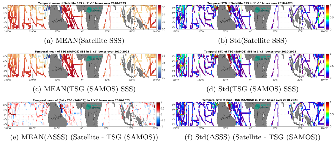
Figure 6: Temporal mean (left) and Std (right) of SSS from SMOS SSS L3 v9 - 9 Days (CATDS-CEC-LOCEAN) (top), TSG (SAMOS) (middle), and of \Delta SSS (Satellite - TSG (SAMOS)). Only match-up pairs are used to generate these maps.
