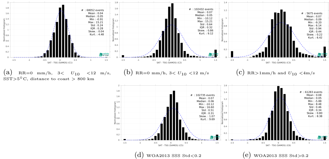
Figure 13: Normalized histogram of \Delta SSS (SMOS SSS L3 v9 - 9 Days (CATDS-CEC-LOCEAN) - TSG (SAMOS)) for 5 different subdatasets corresponding to: RR=0 mm/h, 3 < U_{10} < 12 m/s, SST >5^\circ C, distance to coast > 800 km (a), RR=0 mm/h, 3 < U_{10} < 12 m/s (b), RR >1 mm/h and U_{10} < 4 m/s (c), WOA2013 SSS Std <0.2 (d), WOA2013 SSS Std >0.2 (e).
