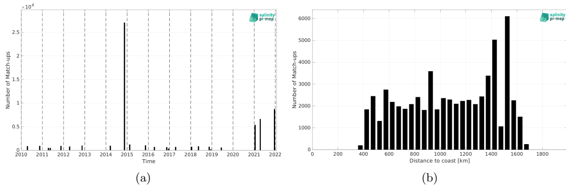
Figure 1: Number of match-ups between TSG (Polarstern) and SMOS SSS L3 v9 - 9 Days (CATDS-CEC-LOCEAN) SSS as a function of time (a) and as function of the distance to coast (b) over the Equatorial Ocean 10N-10S Pi-MEP region and for the full satellite product period.
