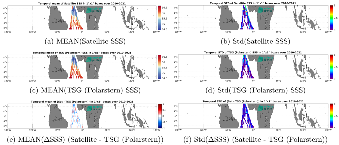
Figure 6: Temporal mean (left) and Std (right) of SSS from SMOS SSS L3 v9 - 9 Days (CATDS-CEC-LOCEAN) (top), TSG (Polarstern) (middle), and of \Delta SSS (Satellite - TSG (Polarstern)). Only match-up pairs are used to generate these maps.
