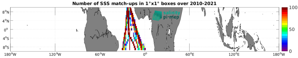
Figure 4: Number of SSS match-ups between TSG (Polarstern) SSS and the SMOS SSS L3 v9 - 9 Days (CATDS-CEC-LOCEAN) SSS product for the Equatorial Ocean 10N-10S Pi-MEP region over 1^\circ \times 1^\circ boxes and for the full satellite product period.
