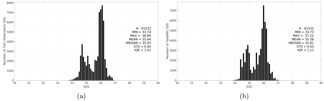
Figure 2: Histograms of SSS from TSG (Polarstern) (a) and SMOS SSS L3 v9 - 9 Days (CATDS-CEC-LOCEAN) (b) considering all match-up pairs per bins of 0.1 over the Equatorial Ocean 10N-10S Pi-MEP region and for the full satellite product period.
