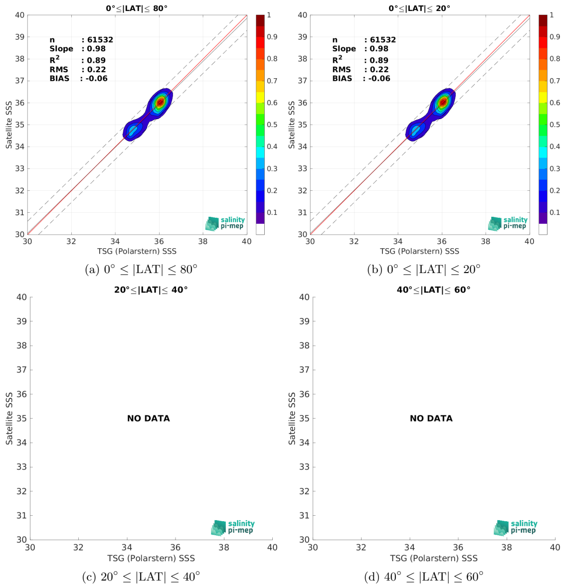
Figure 9: Contour maps of the concentration of SMOS SSS L3 v9 - 9 Days (CATDS-CEC-LOCEAN) SSS (y-axis) versus TSG (Polarstern) SSS (x-axis) at match-up pairs for different latitude bands. For each plot, the red line shows x=y . The black thin and dashed lines indicate a linear fit through the data cloud and the \pm 95\% confidence levels, respectively. The number match-up pairs n , the slope and R^2 coefficient of the linear fit, the root mean square (RMS) and the mean bias between satellite and in situ data are indicated for each latitude band in each plots.
