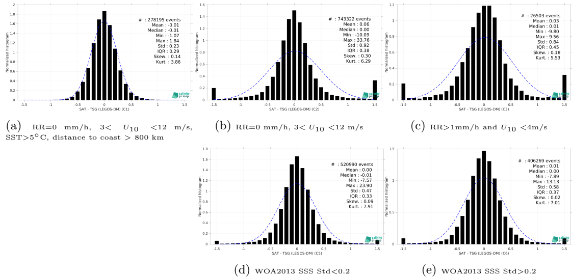
Figure 15: Normalized histogram of \Delta\text{SSS} (SMOS SSS L3 v9 - 9 Days (CATDS-CEC-LOCEAN) - TSG (LEGOS-DM)) for 5 different subdatasets corresponding to: RR=0 mm/h, 3 < U_{10} < 12 m/s, SST>5°C, distance to coast > 800 km (a), RR=0 mm/h, 3 < U_{10} < 12 m/s (b), RR>1mm/h and U_{10} < 4 m/s (c), WOA2013 SSS Std<0.2 (d), WOA2013 SSS Std>0.2 (e).
