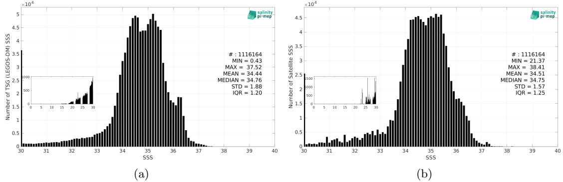
Figure 3: Histograms of SSS from TSG (LEGOS-DM) (a) and SMOS SSS L3 v9 - 9 Days (CATDS-CEC-LOCEAN) (b) considering all match-up pairs per bins of 0.1 over the Equatorial Ocean 10N-10S Pi-MEP region and for the full satellite product period.
