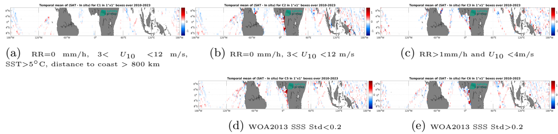
Figure 14: Temporal mean gridded over spatial boxes of size 1^\circ \times 1^\circ of \Delta\text{SSS} (SMOS SSS L3 v9 - 9 Days (CATDS-CEC-LOCEAN) - TSG (LEGOS-DM)) for 5 different subdatasets corresponding to: RR=0 mm/h, 3 < U_{10} < 12 m/s, SST>5°C, distance to coast > 800 km (a), RR=0 mm/h, 3 < U_{10} < 12 m/s (b), RR>1mm/h and U_{10} < 4 m/s (c), WOA2013 SSS Std<0.2 (d), WOA2013 SSS Std>0.2 (e).
