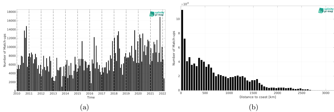
Figure 2: Number of match-ups between TSG (LEGOS-DM) and SMOS SSS L3 v9 - 9 Days (CATDS-CEC-LOCEAN) SSS as a function of time (a) and as function of the distance to coast (b) over the Equatorial Ocean 10N-10S Pi-MEP region and for the full satellite product period.
