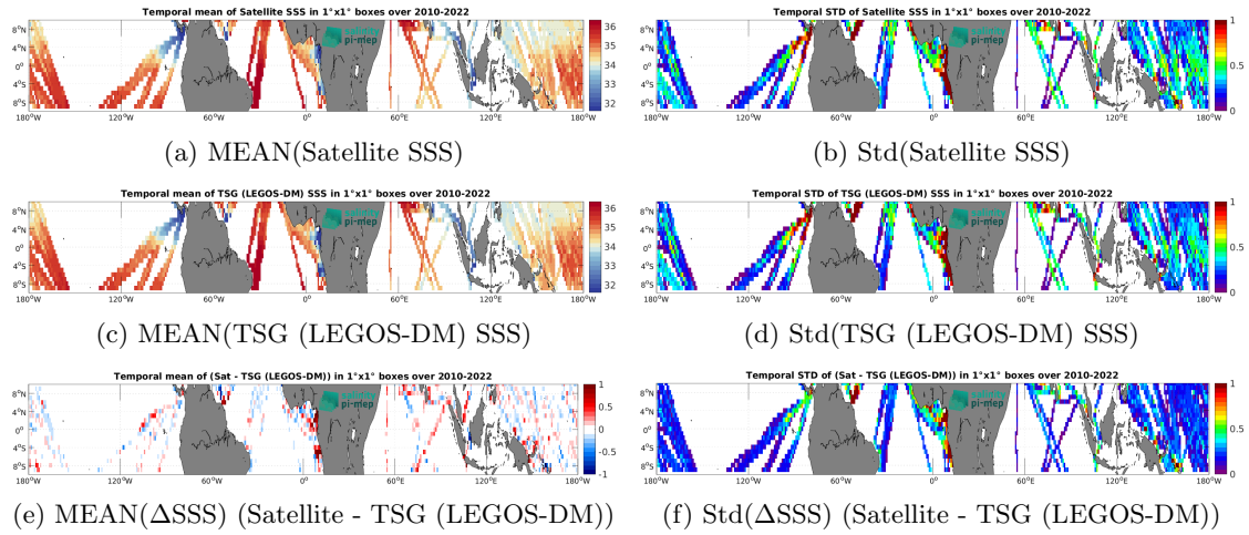
Figure 7: Temporal mean (left) and Std (right) of SSS from SMOS SSS L3 v9 - 9 Days (CATDS-CEC-LOCEAN) (top), TSG (LEGOS-DM) (middle), and of \Delta SSS (Satellite - TSG (LEGOS-DM)). Only match-up pairs are used to generate these maps.
