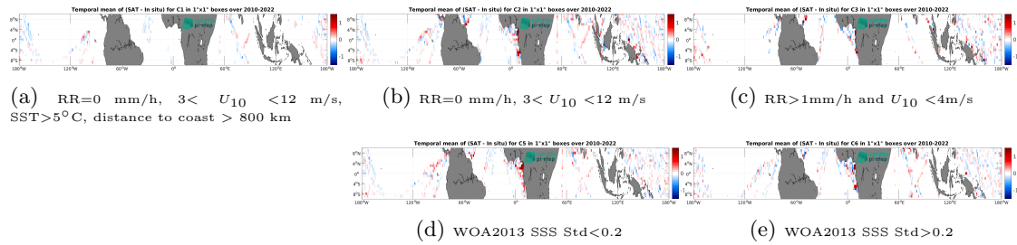
Figure 14: Temporal mean gridded over spatial boxes of size 1^\circ \times 1^\circ of \Delta SSS (SMOS SSS L3 v9 - 9 Days (CATDS-CEC-LOCEAN) - TSG (LEGOS-DM)) for 5 different subdatasets corresponding to: RR=0 mm/h, 3 < U_{10} < 12 m/s, SST>5°C, distance to coast > 800 km (a), RR=0 mm/h, 3 < U_{10} < 12 m/s (b), RR>1mm/h and U_{10} < 4 m/s (c), WOA2013 SSS Std<0.2 (d), WOA2013 SSS Std>0.2 (e).
