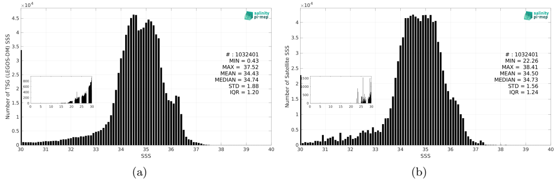
Figure 3: Histograms of SSS from TSG (LEGOS-DM) (a) and SMOS SSS L3 v9 - 9 Days (CATDS-CEC-LOCEAN) (b) considering all match-up pairs per bins of 0.1 over the Equatorial Ocean 10N-10S Pi-MEP region and for the full satellite product period.
