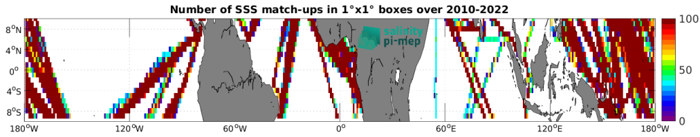
Figure 5: Number of SSS match-ups between TSG (LEGOS-DM) SSS and the SMOS SSS L3 v9 - 9 Days (CATDS-CEC-LOCEAN) SSS product for the Equatorial Ocean 10N-10S Pi-MEP region over 1^\circ \times 1^\circ boxes and for the full satellite product period.
