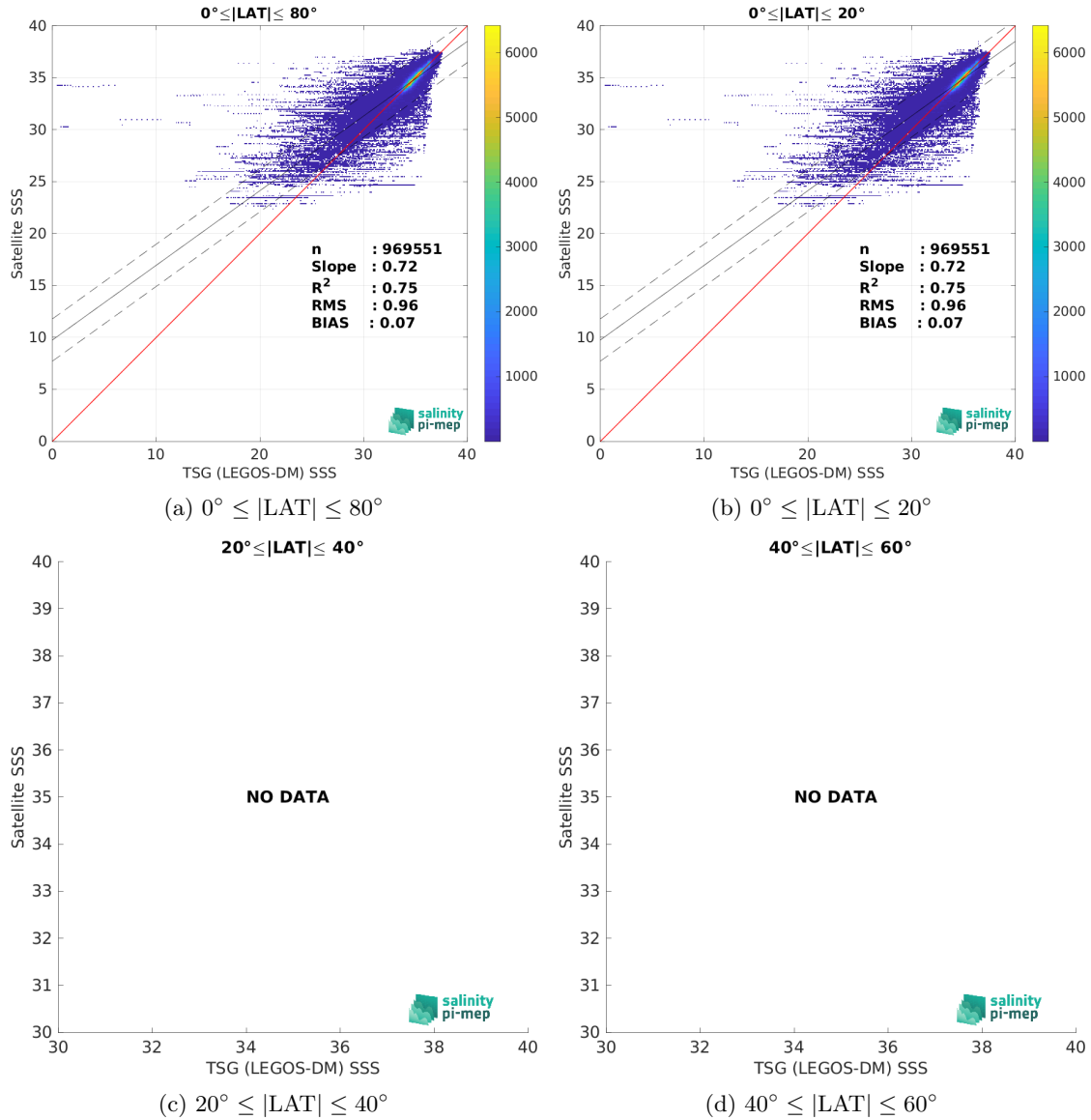
Figure 9: Contour maps of the concentration of SMOS SSS L3 v9 - 9 Days (CATDS-CEC-LOCEAN) SSS (y-axis) versus TSG (LEGOS-DM) SSS (x-axis) at match-up pairs for different latitude bands. For each plot, the red line shows x=y . The black thin and dashed lines indicate a linear fit through the data cloud and the \pm 95\% confidence levels, respectively. The number match-up pairs n , the slope and R^2 coefficient of the linear fit, the root mean square (RMS) and the mean bias between satellite and in situ data are indicated for each latitude band in each plots.
