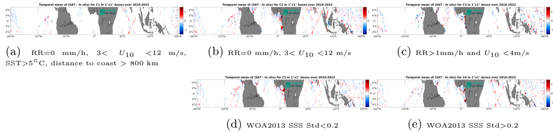
Figure 12: Temporal mean gridded over spatial boxes of size 1^\circ \times 1^\circ of \Delta SSS (SMOS SSS L3 v9 - 9 Days (CATDS-CEC-LOCEAN) - TSG (LEGOS-DM)) for 5 different subdatasets corresponding to: RR=0 mm/h, 3 < U_{10} < 12 m/s, SST >5^\circ C, distance to coast > 800 km (a), RR=0 mm/h, 3 < U_{10} < 12 m/s (b), RR >1 mm/h and U_{10} < 4 m/s (c), WOA2013 SSS Std <0.2 (d), WOA2013 SSS Std >0.2 (e).
