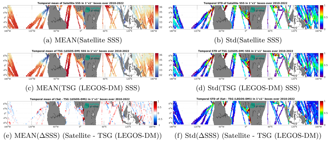
Figure 6: Temporal mean (left) and Std (right) of SSS from SMOS SSS L3 v9 - 9 Days (CATDS-CEC-LOCEAN) (top), TSG (LEGOS-DM) (middle), and of \Delta SSS (Satellite - TSG (LEGOS-DM)). Only match-up pairs are used to generate these maps.
