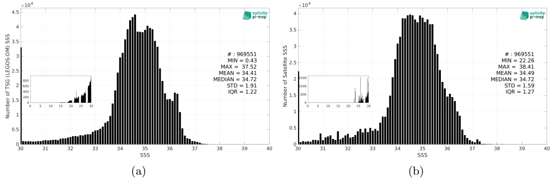
Figure 2: Histograms of SSS from TSG (LEGOS-DM) (a) and SMOS SSS L3 v9 - 9 Days (CATDS-CEC-LOCEAN) (b) considering all match-up pairs per bins of 0.1 over the Equatorial Ocean 10N-10S Pi-MEP region and for the full satellite product period.
