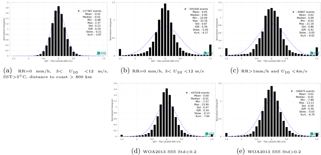
Figure 13: Normalized histogram of \Delta SSS (SMOS SSS L3 v9 - 9 Days (CATDS-CEC-LOCEAN) - TSG (LEGOS-DM)) for 5 different subdatasets corresponding to: RR=0 mm/h, 3 < U_{10} < 12 m/s, SST >5^\circ C, distance to coast > 800 km (a), RR=0 mm/h, 3 < U_{10} < 12 m/s (b), RR >1 mm/h and U_{10} < 4 m/s (c), WOA2013 SSS Std <0.2 (d), WOA2013 SSS Std >0.2 (e).
