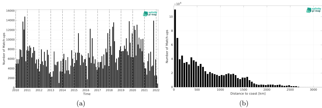
Figure 1: Number of match-ups between TSG (LEGOS-DM) and SMOS SSS L3 v9 - 9 Days (CATDS-CEC-LOCEAN) SSS as a function of time (a) and as function of the distance to coast (b) over the Equatorial Ocean 10N-10S Pi-MEP region and for the full satellite product period.
