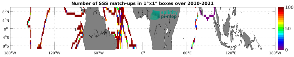
Figure 5: Number of SSS match-ups between TSG (GOSUD-Sailing-ship) SSS and the SMOS SSS L3 v9 - 9 Days (CATDS-CEC-LOCEAN) SSS product for the Equatorial Ocean 10N-10S Pi-MEP region over 1^\circ \times 1^\circ boxes and for the full satellite product period.
