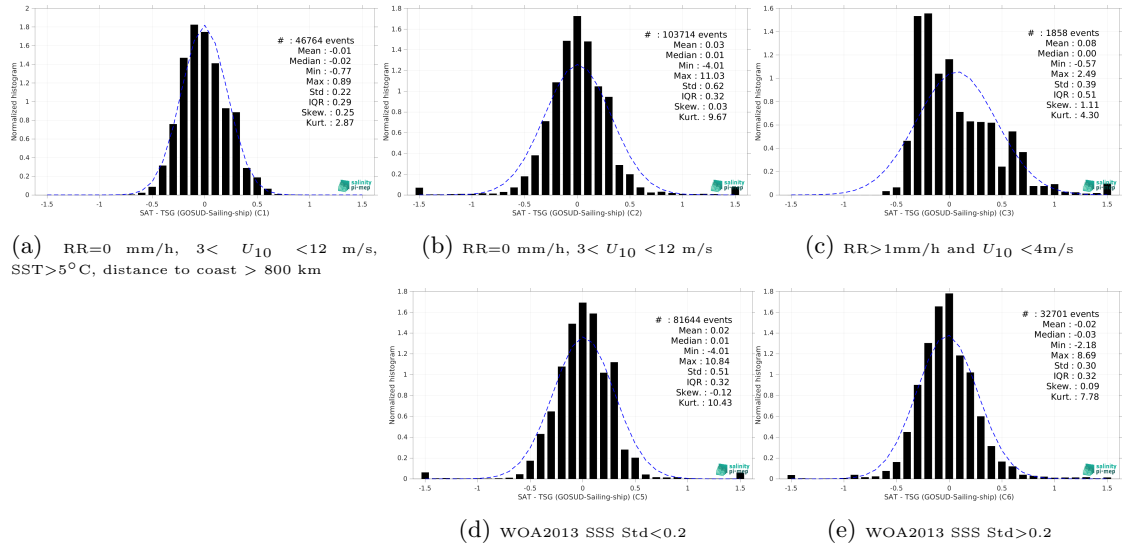
Figure 15: Normalized histogram of \Delta\text{SSS} (SMOS SSS L3 v9 - 9 Days (CATDS-CEC-LOCEAN) - TSG (GOSUD-Sailing-ship)) for 5 different subdatasets corresponding to: RR=0 mm/h, 3 < U_{10} < 12 m/s, SST>5°C, distance to coast > 800 km (a), RR=0 mm/h, 3 < U_{10} < 12 m/s (b), RR>1mm/h and U_{10} < 4 m/s (c), WOA2013 SSS Std<0.2 (d), WOA2013 SSS Std>0.2 (e).
