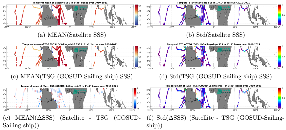
Figure 7: Temporal mean (left) and Std (right) of SSS from SMOS SSS L3 v9 - 9 Days (CATDS-CEC-LOCEAN) (top), TSG (GOSUD-Sailing-ship) (middle), and of \Delta SSS (Satellite - TSG (GOSUD-Sailing-ship)). Only match-up pairs are used to generate these maps.
