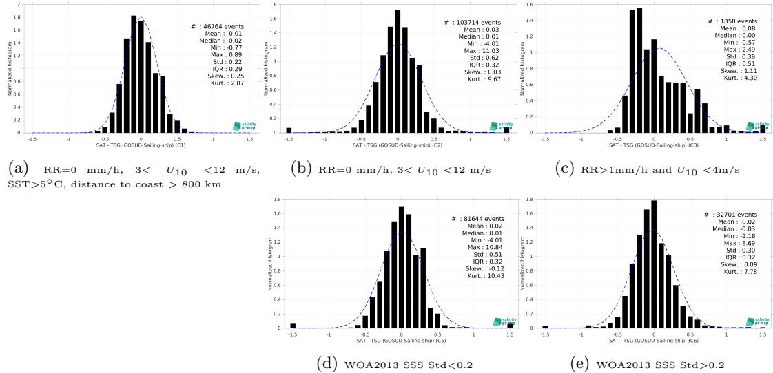
Figure 15: Normalized histogram of \Delta\text{SSS} (SMOS SSS L3 v9 - 9 Days (CATDS-CEC-LOCEAN) - TSG (GOSUD-Sailing-ship)) for 5 different subdatasets corresponding to: RR=0 mm/h, 3 < U_{10} < 12 m/s, SST>5°C, distance to coast > 800 km (a), RR=0 mm/h, 3 < U_{10} < 12 m/s (b), RR>1mm/h and U_{10} < 4 m/s (c), WOA2013 SSS Std<0.2 (d), WOA2013 SSS Std>0.2 (e).
