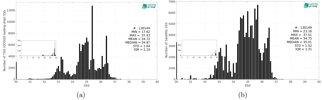
Figure 2: Histograms of SSS from TSG (GOSUD-Sailing-ship) (a) and SMOS SSS L3 v9 - 9 Days (CATDS-CEC-LOCEAN) (b) considering all match-up pairs per bins of 0.1 over the Equatorial Ocean 10N-10S Pi-MEP region and for the full satellite product period.
