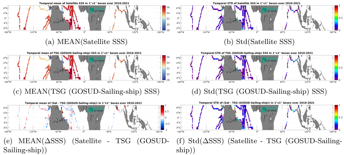
Figure 6: Temporal mean (left) and Std (right) of SSS from SMOS SSS L3 v9 - 9 Days (CATDS-CEC-LOCEAN) (top), TSG (GOSUD-Sailing-ship) (middle), and of \Delta SSS (Satellite - TSG (GOSUD-Sailing-ship)). Only match-up pairs are used to generate these maps.
