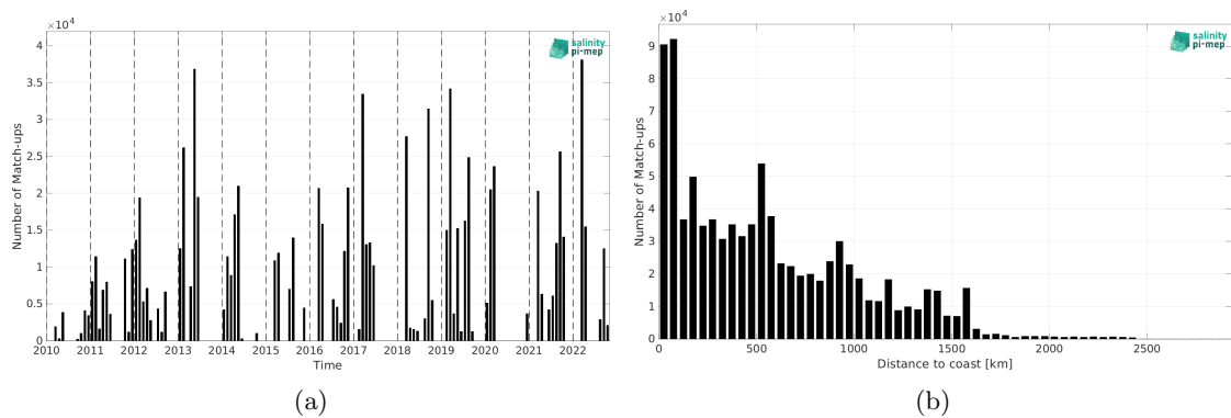
Figure 2: Number of match-ups between TSG (GOSUD-Research-vessel) and SMOS SSS L3 v9 - 9 Days (CATDS-CEC-LOCEAN) SSS as a function of time (a) and as function of the distance to coast (b) over the Equatorial Ocean 10N-10S Pi-MEP region and for the full satellite product period.
