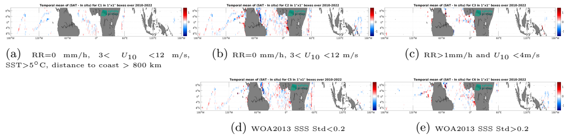
Figure 14: Temporal mean gridded over spatial boxes of size 1^\circ \times 1^\circ of \Delta\text{SSS} (SMOS SSS L3 v9 - 9 Days (CATDS-CEC-LOCEAN) - TSG (GOSUD-Research-vessel)) for 5 different subdatasets corresponding to: RR=0 mm/h, 3 < U_{10} < 12 m/s, SST>5°C, distance to coast > 800 km (a), RR=0 mm/h, 3 < U_{10} < 12 m/s (b), RR>1mm/h and U_{10} < 4 m/s (c), WOA2013 SSS Std<0.2 (d), WOA2013 SSS Std>0.2 (e).
