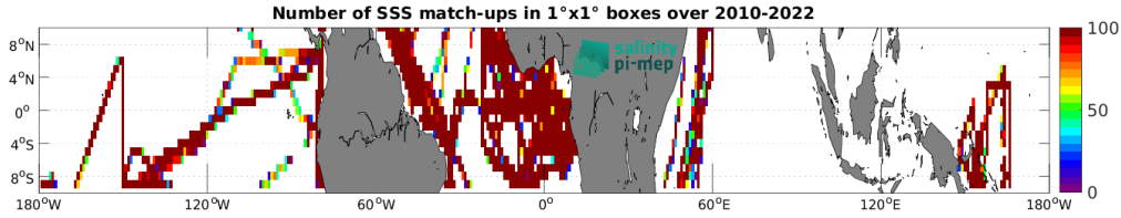
Figure 5: Number of SSS match-ups between TSG (GOSUD-Research-vessel) SSS and the SMOS SSS L3 v9 - 9 Days (CATDS-CEC-LOCEAN) SSS product for the Equatorial Ocean 10N-10S Pi-MEP region over 1^\circ \times 1^\circ boxes and for the full satellite product period.
