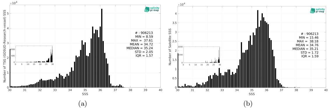
Figure 3: Histograms of SSS from TSG (GOSUD-Research-vessel) (a) and SMOS SSS L3 v9 - 9 Days (CATDS-CEC-LOCEAN) (b) considering all match-up pairs per bins of 0.1 over the Equatorial Ocean 10N-10S Pi-MEP region and for the full satellite product period.
