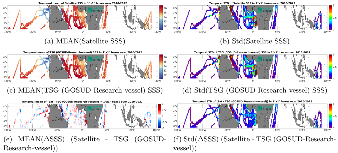
Figure 7: Temporal mean (left) and Std (right) of SSS from SMOS SSS L3 v9 - 9 Days (CATDS-CEC-LOCEAN) (top), TSG (GOSUD-Research-vessel) (middle), and of \Delta SSS (Satellite - TSG (GOSUD-Research-vessel)). Only match-up pairs are used to generate these maps.
