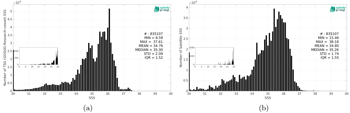
Figure 3: Histograms of SSS from TSG (GOSUD-Research-vessel) (a) and SMOS SSS L3 v9 - 9 Days (CATDS-CEC-LOCEAN) (b) considering all match-up pairs per bins of 0.1 over the Equatorial Ocean 10N-10S Pi-MEP region and for the full satellite product period.
