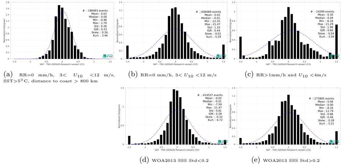
Figure 13: Normalized histogram of \Delta\text{SSS} (SMOS SSS L3 v9 - 9 Days (CATDS-CEC-LOCEAN) - TSG (GOSUD-Research-vessel)) for 5 different subdatasets corresponding to: RR=0 mm/h, 3 < U_{10} < 12 m/s, SST>5°C, distance to coast > 800 km (a), RR=0 mm/h, 3 < U_{10} < 12 m/s (b), RR>1mm/h and U_{10} < 4 m/s (c), WOA2013 SSS Std<0.2 (d), WOA2013 SSS Std>0.2 (e).
