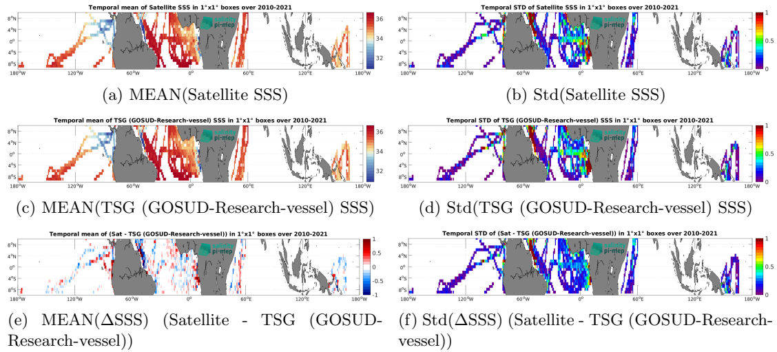
Figure 6: Temporal mean (left) and Std (right) of SSS from SMOS SSS L3 v9 - 9 Days (CATDS-CEC-LOCEAN) (top), TSG (GOSUD-Research-vessel) (middle), and of \Delta SSS (Satellite - TSG (GOSUD-Research-vessel)). Only match-up pairs are used to generate these maps.
