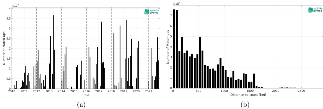
Figure 1: Number of match-ups between TSG (GOSUD-Research-vessel) and SMOS SSS L3 v9 - 9 Days (CATDS-CEC-LOCEAN) SSS as a function of time (a) and as function of the distance to coast (b) over the Equatorial Ocean 10N-10S Pi-MEP region and for the full satellite product period.
