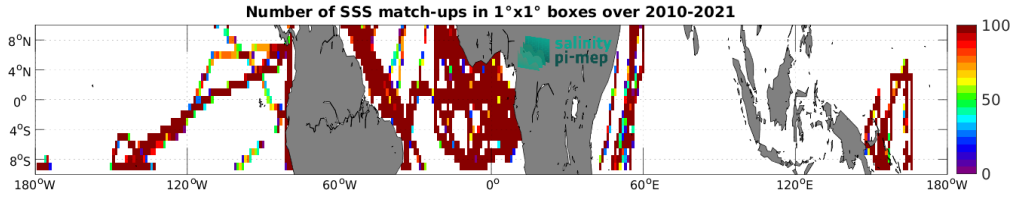
Figure 4: Number of SSS match-ups between TSG (GOSUD-Research-vessel) SSS and the SMOS SSS L3 v9 - 9 Days (CATDS-CEC-LOCEAN) SSS product for the Equatorial Ocean 10N-10S Pi-MEP region over 1^\circ \times 1^\circ boxes and for the full satellite product period.
