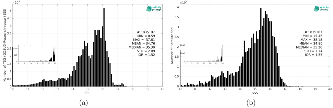
Figure 2: Histograms of SSS from TSG (GOSUD-Research-vessel) (a) and SMOS SSS L3 v9 - 9 Days (CATDS-CEC-LOCEAN) (b) considering all match-up pairs per bins of 0.1 over the Equatorial Ocean 10N-10S Pi-MEP region and for the full satellite product period.
