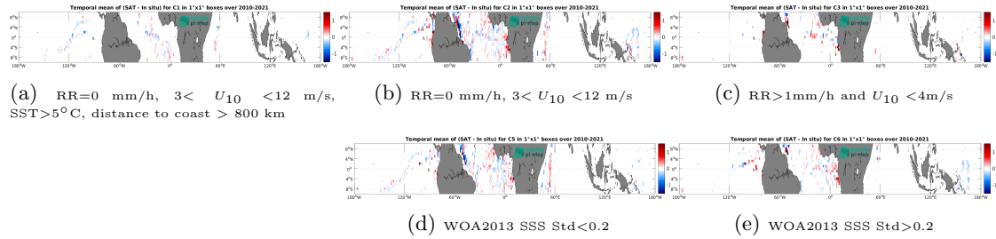
Figure 12: Temporal mean gridded over spatial boxes of size 1^\circ \times 1^\circ of \Delta\text{SSS} (SMOS SSS L3 v9 - 9 Days (CATDS-CEC-LOCEAN) - TSG (GOSUD-Research-vessel)) for 5 different subdatasets corresponding to:RR=0 mm/h, 3 < U_{10} < 12 m/s, SST>5°C, distance to coast > 800 km (a), RR=0 mm/h, 3 < U_{10} < 12 m/s (b), RR>1mm/h and U_{10} < 4 m/s (c), WOA2013 SSS Std<0.2 (d), WOA2013 SSS Std>0.2 (e).
