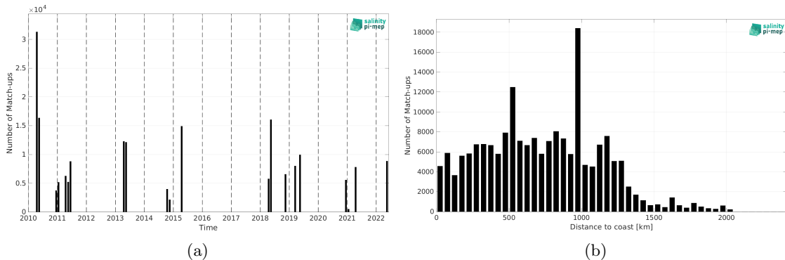
Figure 2: Number of match-ups between TSG (CSIC-UTM) and SMOS SSS L3 v9 - 9 Days (CATDS-CEC-LOCEAN) SSS as a function of time (a) and as function of the distance to coast (b) over the Equatorial Ocean 10N-10S Pi-MEP region and for the full satellite product period.
