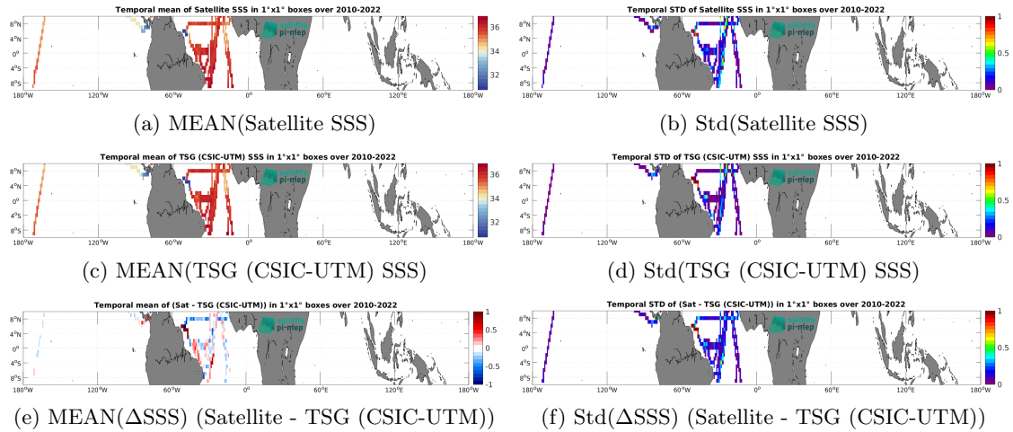
Figure 7: Temporal mean (left) and Std (right) of SSS from SMOS SSS L3 v9 - 9 Days (CATDS-CEC-LOCEAN) (top), TSG (CSIC-UTM) (middle), and of \Delta SSS (Satellite - TSG (CSIC-UTM)). Only match-up pairs are used to generate these maps.
