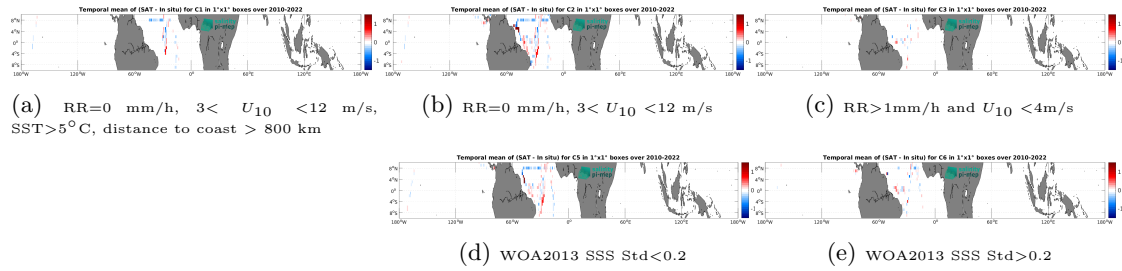
Figure 12: Temporal mean gridded over spatial boxes of size 1^\circ \times 1^\circ of \Delta SSS (SMOS SSS L3 v9 - 9 Days (CATDS-CEC-LOCEAN) - TSG (CSIC-UTM)) for 5 different subdatasets corresponding to: RR=0 mm/h, 3 < U_{10} < 12 m/s, SST >5^\circ\text{C} , distance to coast > 800 km (a), RR=0 mm/h, 3 < U_{10} < 12 m/s (b), RR >1 mm/h and U_{10} < 4 m/s (c), WOA2013 SSS Std <0.2 (d), WOA2013 SSS Std >0.2 (e).
