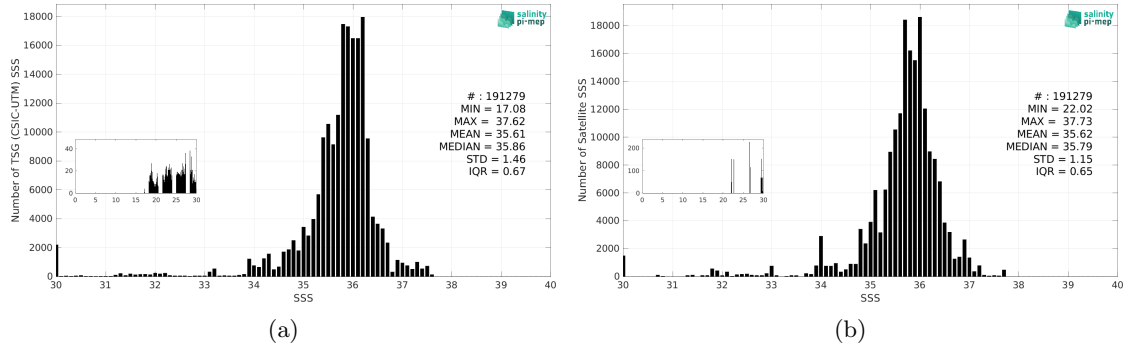
Figure 2: Histograms of SSS from TSG (CSIC-UTM) (a) and SMOS SSS L3 v9 - 9 Days (CATDS-CEC-LOCEAN) (b) considering all match-up pairs per bins of 0.1 over the Equatorial Ocean 10N-10S Pi-MEP region and for the full satellite product period.
