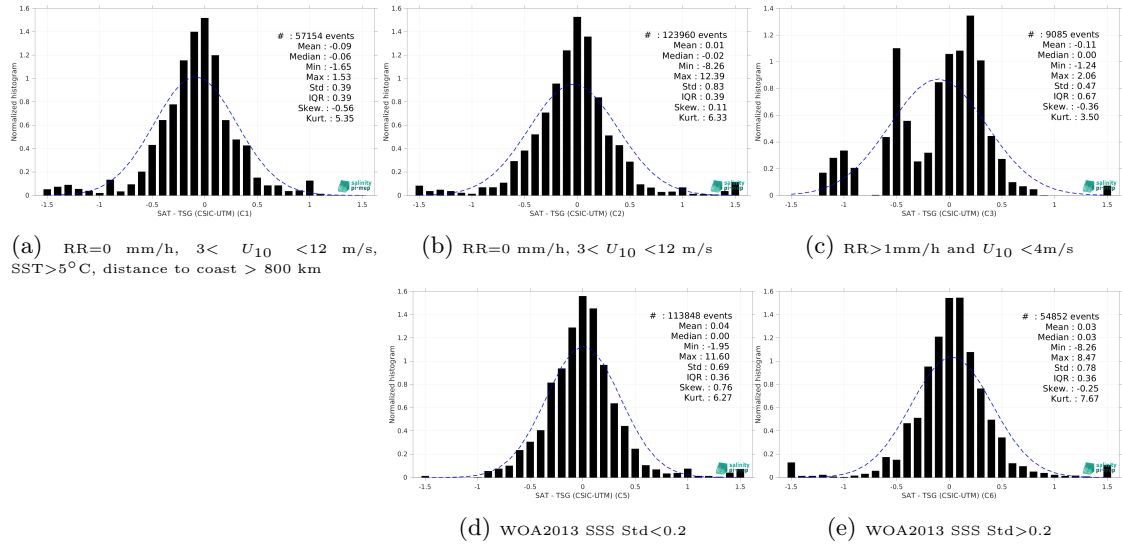
Figure 13: Normalized histogram of \Delta SSS (SMOS SSS L3 v9 - 9 Days (CATDS-CEC-LOCEAN) - TSG (CSIC-UTM)) for 5 different subdatasets corresponding to: RR=0 mm/h, 3 < U_{10} < 12 m/s, SST >5^\circ\text{C} , distance to coast > 800 km (a), RR=0 mm/h, 3 < U_{10} < 12 m/s (b), RR >1 mm/h and U_{10} < 4 m/s (c), WOA2013 SSS Std <0.2 (d), WOA2013 SSS Std >0.2 (e).
