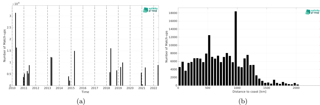
Figure 1: Number of match-ups between TSG (CSIC-UTM) and SMOS SSS L3 v9 - 9 Days (CATDS-CEC-LOCEAN) SSS as a function of time (a) and as function of the distance to coast (b) over the Equatorial Ocean 10N-10S Pi-MEP region and for the full satellite product period.
