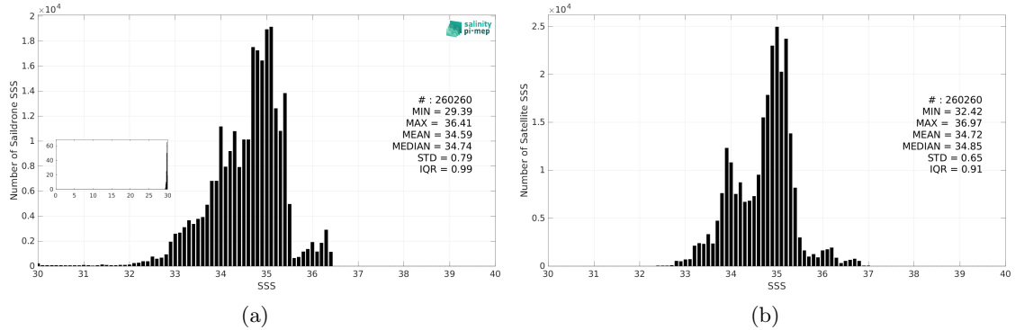
Figure 3: Histograms of SSS from Saildrone (a) and SMOS SSS L3 v9 - 9 Days (CATDS-CEC-LOCEAN) (b) considering all match-up pairs per bins of 0.1 over the Equatorial Ocean 10N-10S Pi-MEP region and for the full satellite product period.
