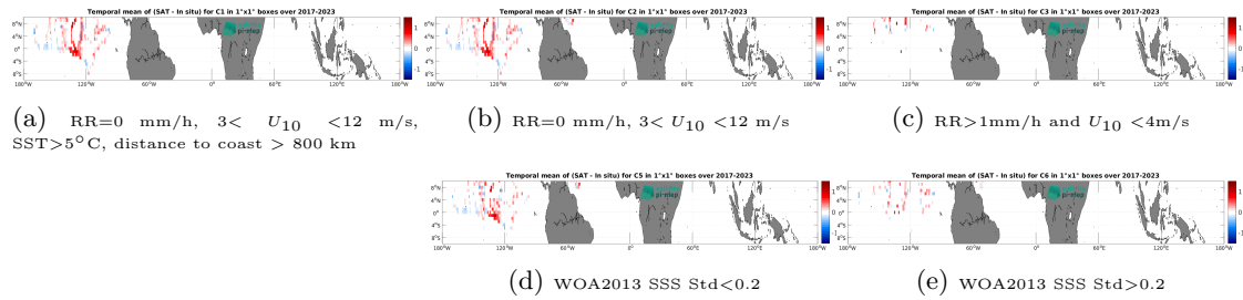
Figure 14: Temporal mean gridded over spatial boxes of size 1^\circ \times 1^\circ of \Delta SSS (SMOS SSS L3 v9 - 9 Days (CATDS-CEC-LOCEAN) - Saildrone) for 5 different subdatasets corresponding to: RR=0 mm/h, 3 < U_{10} < 12 m/s, SST>5°C, distance to coast > 800 km (a), RR=0 mm/h, 3 < U_{10} < 12 m/s (b), RR>1mm/h and U_{10} < 4 m/s (c), WOA2013 SSS Std<0.2 (d), WOA2013 SSS Std>0.2 (e).
