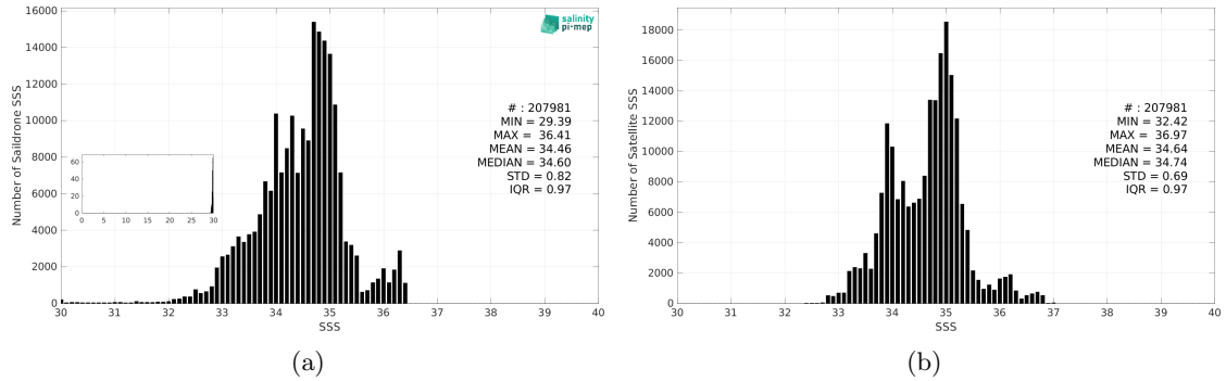
Figure 3: Histograms of SSS from Saildrone (a) and SMOS SSS L3 v9 - 9 Days (CATDS-CEC-LOCEAN) (b) considering all match-up pairs per bins of 0.1 over the Equatorial Ocean 10N-10S Pi-MEP region and for the full satellite product period.
