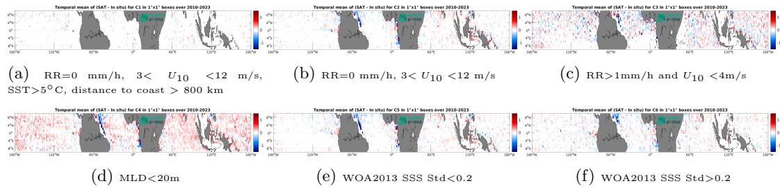
Figure 12: Temporal mean gridded over spatial boxes of size 1^\circ \times 1^\circ of \Delta SSS (SMOS SSS L3 v9 - 9 Days (CATDS-CEC-LOCEAN) - Argo) for 6 different subdatasets corresponding to:RR=0 mm/h, 3 < U_{10} < 12 m/s, SST >5^\circ C, distance to coast > 800 km (a), RR=0 mm/h, 3 < U_{10} < 12 m/s (b), RR >1 mm/h and U_{10} < 4 m/s (c),MLD <20 m (d),WOA2013 SSS Std <0.2 (e),WOA2013 SSS Std >0.2 (f).
