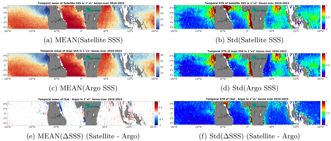
Figure 6: Temporal mean (left) and Std (right) of SSS from SMOS SSS L3 v9 - 9 Days (CATDS-CEC-LOCEAN) (top), Argo (middle), and of \Delta SSS (Satellite - Argo). Only match-up pairs are used to generate these maps.
