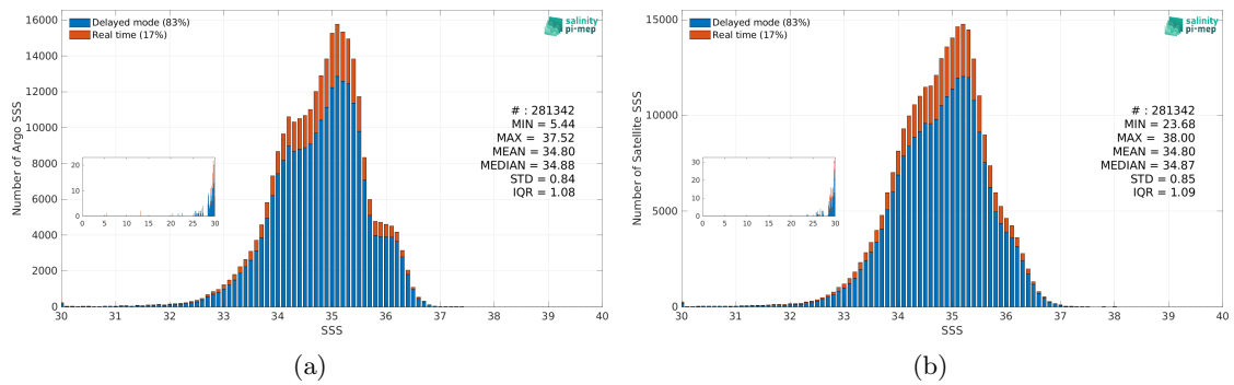
Figure 2: Histograms of SSS from Argo (a) and SMOS SSS L3 v9 - 9 Days (CATDS-CEC-LOCEAN) (b) considering all match-up pairs per bins of 0.1 over the Equatorial Ocean 10N-10S Pi-MEP region and for the full satellite product period.
