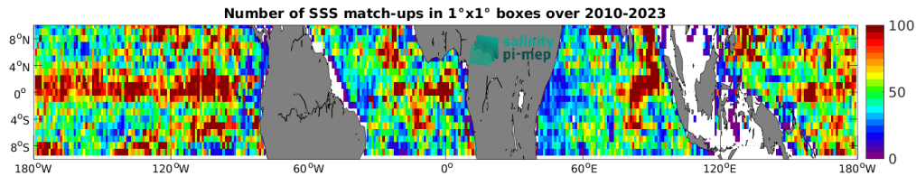
Figure 4: Number of SSS match-ups between Argo SSS and the SMOS SSS L3 v9 - 9 Days (CATDS-CEC-LOCEAN) SSS product for the Equatorial Ocean 10N-10S Pi-MEP region over 1^\circ \times 1^\circ boxes and for the full satellite product period.
