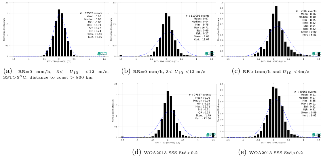
Figure 15: Normalized histogram of \Delta SSS (SMOS SSS L3 v9 - 18 Days (CATDS-CEC-LOCEAN) - TSG (SAMOS)) for 5 different subdatasets corresponding to: RR=0 mm/h, 3 < U_{10} < 12 m/s, SST> 5^\circ C, distance to coast > 800 km (a), RR=0 mm/h, 3 < U_{10} < 12 m/s (b), RR>1mm/h and U_{10} < 4 m/s (c), WOA2013 SSS Std<0.2 (d), WOA2013 SSS Std>0.2 (e).
