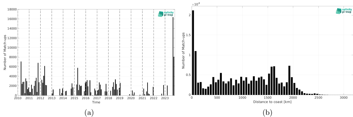
Figure 1: Number of match-ups between TSG (SAMOS) and SMOS SSS L3 v9 - 18 Days (CATDS-CEC-LOCEAN) SSS as a function of time (a) and as function of the distance to coast (b) over the Equatorial Ocean 10N-10S Pi-MEP region and for the full satellite product period.
