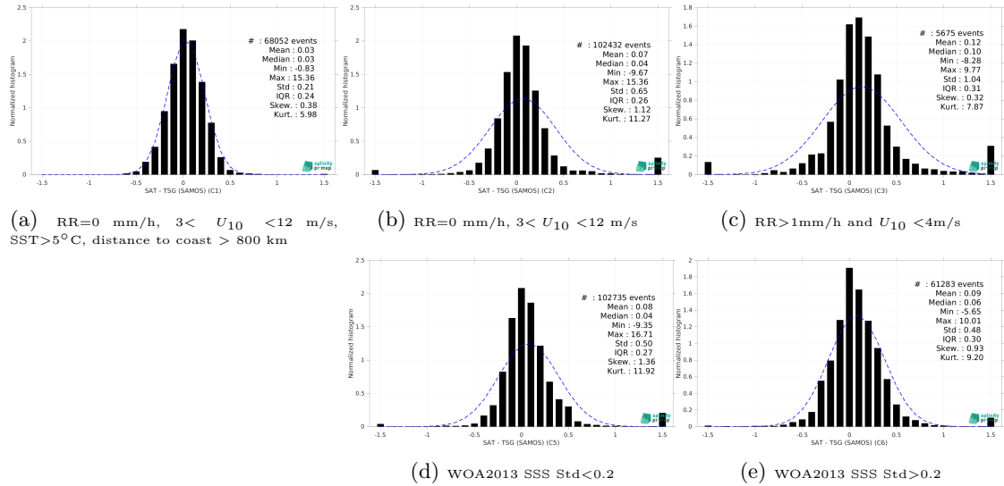
Figure 13: Normalized histogram of \Delta SSS (SMOS SSS L3 v9 - 18 Days (CATDS-CEC-LOCEAN) - TSG (SAMOS)) for 5 different subdatasets corresponding to: RR=0 mm/h, 3 < U_{10} < 12 m/s, SST >5^\circ C, distance to coast > 800 km (a), RR=0 mm/h, 3 < U_{10} < 12 m/s (b), RR >1 mm/h and U_{10} < 4 m/s (c), WOA2013 SSS Std <0.2 (d), WOA2013 SSS Std >0.2 (e).
