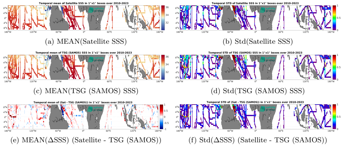
Figure 6: Temporal mean (left) and Std (right) of SSS from SMOS SSS L3 v9 - 18 Days (CATDS-CEC-LOCEAN) (top), TSG (SAMOS) (middle), and of \Delta SSS (Satellite - TSG (SAMOS)). Only match-up pairs are used to generate these maps.
