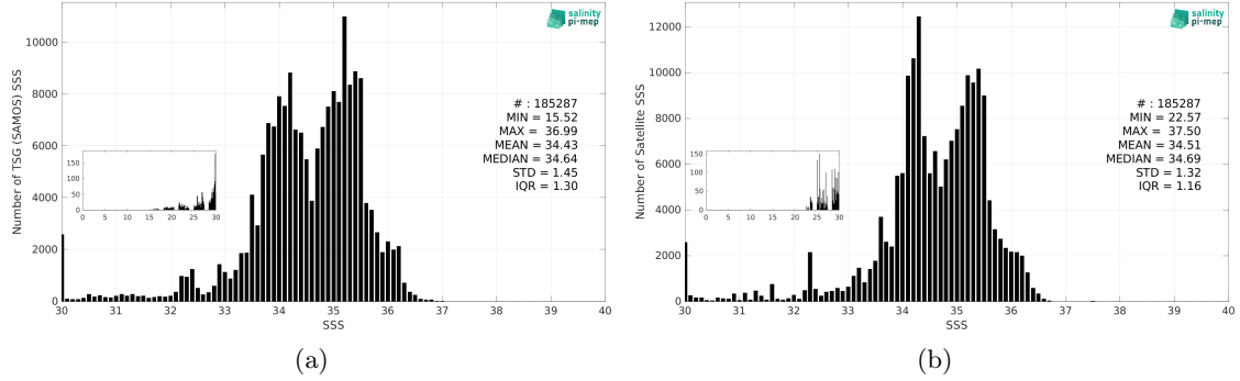
Figure 2: Histograms of SSS from TSG (SAMOS) (a) and SMOS SSS L3 v9 - 18 Days (CATDS-CEC-LOCEAN) (b) considering all match-up pairs per bins of 0.1 over the Equatorial Ocean 10N-10S Pi-MEP region and for the full satellite product period.
