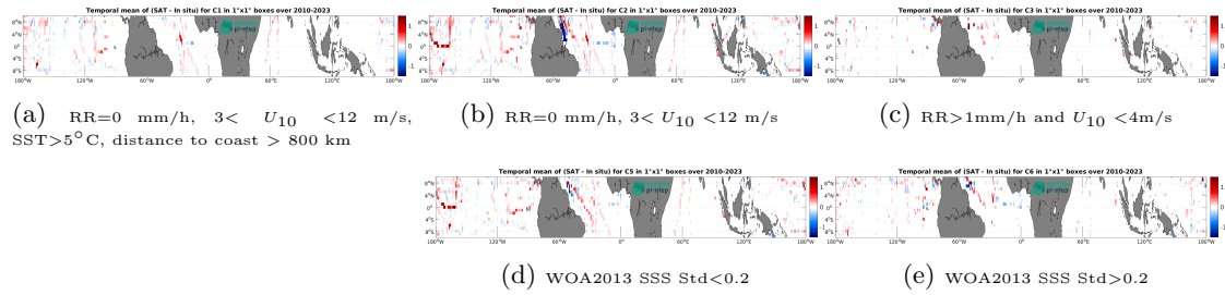
Figure 12: Temporal mean gridded over spatial boxes of size 1^\circ \times 1^\circ of \Delta SSS (SMOS SSS L3 v9 - 18 Days (CATDS-CEC-LOCEAN) - TSG (SAMOS)) for 5 different subdatasets corresponding to: RR=0 mm/h, 3 < U_{10} < 12 m/s, SST >5^\circ C, distance to coast > 800 km (a), RR=0 mm/h, 3 < U_{10} < 12 m/s (b), RR >1 mm/h and U_{10} < 4 m/s (c), WOA2013 SSS Std <0.2 (d), WOA2013 SSS Std >0.2 (e).
