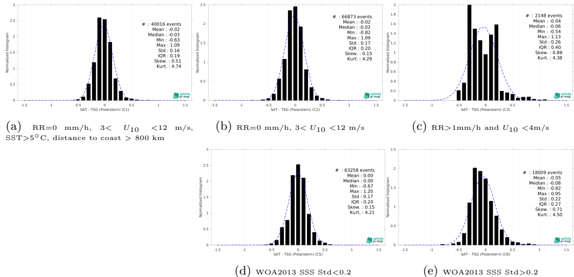
Figure 15: Normalized histogram of \Delta SSS (SMOS SSS L3 v9 - 18 Days (CATDS-CEC-LOCEAN) - TSG (Polarstern)) for 5 different subdatasets corresponding to: RR=0 mm/h, 3 < U_{10} < 12 m/s, SST>5°C, distance to coast > 800 km (a), RR=0 mm/h, 3 < U_{10} < 12 m/s (b), RR>1mm/h and U_{10} < 4 m/s (c), WOA2013 SSS Std<0.2 (d), WOA2013 SSS Std>0.2 (e).
