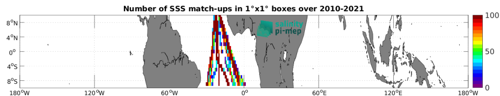
Figure 4: Number of SSS match-ups between TSG (Polarstern) SSS and the SMOS SSS L3 v9 - 18 Days (CATDS-CEC-LOCEAN) SSS product for the Equatorial Ocean 10N-10S Pi-MEP region over 1^\circ \times 1^\circ boxes and for the full satellite product period.
