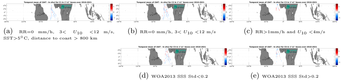
Figure 12: Temporal mean gridded over spatial boxes of size 1^{\circ}\times 1^{\circ} of \Delta\text{SSS} (SMOS SSS L3 v9 - 18 Days (CATDS-CEC-LOCEAN) - TSG (Polarstern)) for 5 different subdatasets corresponding to:RR=0 mm/h, 3 < U_{10} < 12 m/s, SST >5^{\circ}\text{C} , distance to coast > 800 km (a), RR=0 mm/h, 3 < U_{10} < 12 m/s (b), RR >1 mm/h and U_{10} < 4 m/s (c), WOA2013 SSS Std <0.2 (d), WOA2013 SSS Std >0.2 (e).
