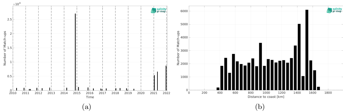
Figure 1: Number of match-ups between TSG (Polarstern) and SMOS SSS L3 v9 - 18 Days (CATDS-CEC-LOCEAN) SSS as a function of time (a) and as function of the distance to coast (b) over the Equatorial Ocean 10N-10S Pi-MEP region and for the full satellite product period.
