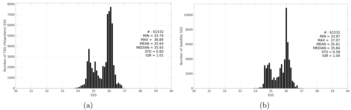
Figure 2: Histograms of SSS from TSG (Polarstern) (a) and SMOS SSS L3 v9 - 18 Days (CATDS-CEC-LOCEAN) (b) considering all match-up pairs per bins of 0.1 over the Equatorial Ocean 10N-10S Pi-MEP region and for the full satellite product period.
