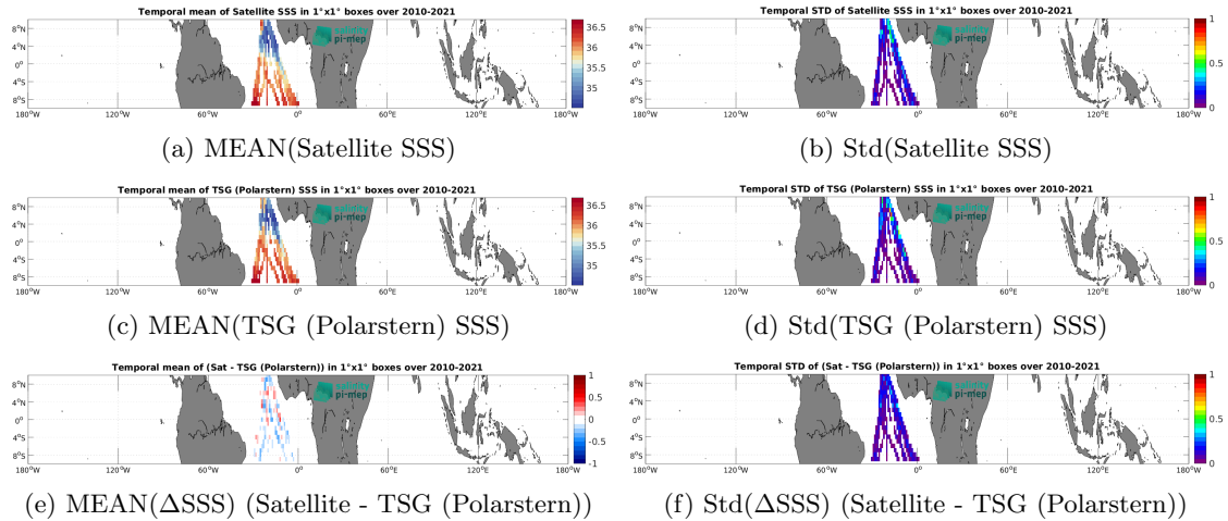
Figure 6: Temporal mean (left) and Std (right) of SSS from SMOS SSS L3 v9 - 18 Days (CATDS-CEC-LOCEAN) (top), TSG (Polarstern) (middle), and of \Delta SSS (Satellite - TSG (Polarstern)). Only match-up pairs are used to generate these maps.
