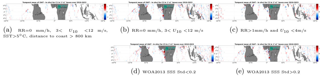
Figure 14: Temporal mean gridded over spatial boxes of size 1^\circ \times 1^\circ of \Delta\text{SSS} (SMOS SSS L3 v9 - 18 Days (CATDS-CEC-LOCEAN) - TSG (LEGOS-DM)) for 5 different subdatasets corresponding to: RR=0 mm/h, 3 < U_{10} < 12 m/s, SST>5°C, distance to coast > 800 km (a), RR=0 mm/h, 3 < U_{10} < 12 m/s (b), RR>1mm/h and U_{10} < 4 m/s (c), WOA2013 SSS Std<0.2 (d), WOA2013 SSS Std>0.2 (e).
