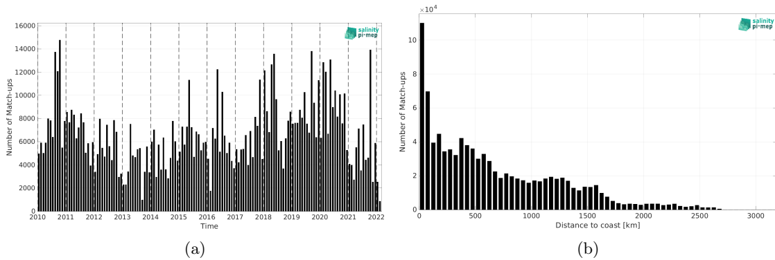
Figure 1: Number of match-ups between TSG (LEGOS-DM) and SMOS SSS L3 v9 - 18 Days (CATDS-CEC-LOCEAN) SSS as a function of time (a) and as function of the distance to coast (b) over the Equatorial Ocean 10N-10S Pi-MEP region and for the full satellite product period.
