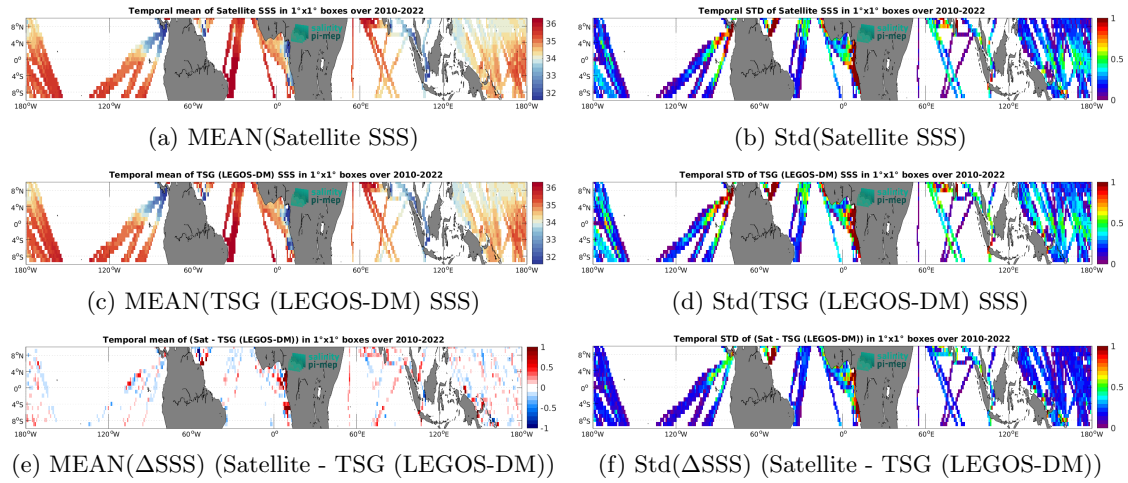
Figure 6: Temporal mean (left) and Std (right) of SSS from SMOS SSS L3 v9 - 18 Days (CATDS-CEC-LOCEAN) (top), TSG (LEGOS-DM) (middle), and of \Delta SSS (Satellite - TSG (LEGOS-DM)). Only match-up pairs are used to generate these maps.
