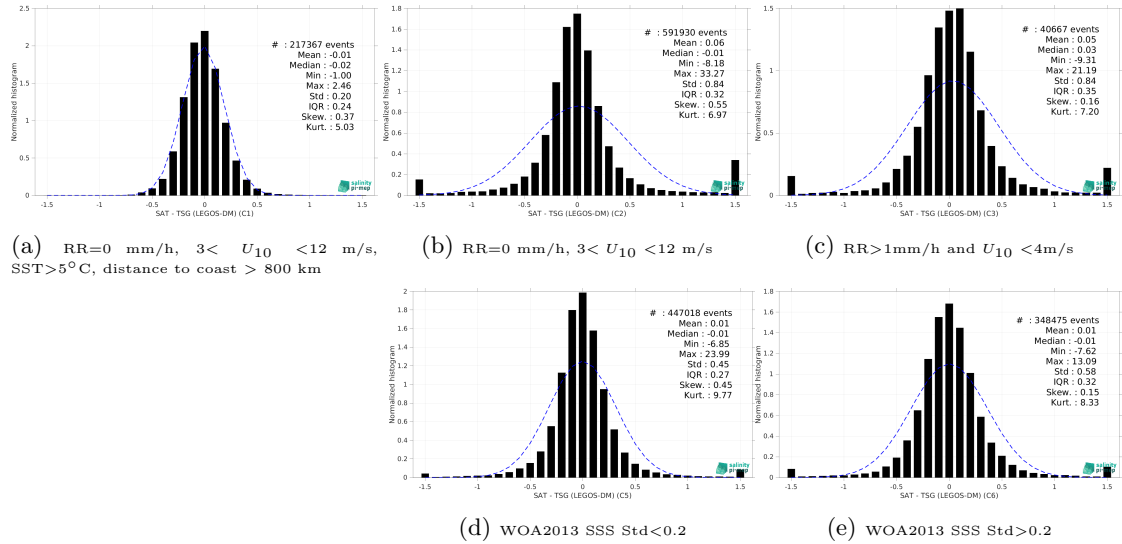
Figure 13: Normalized histogram of \Delta SSS (SMOS SSS L3 v9 - 18 Days (CATDS-CEC-LOCEAN) - TSG (LEGOS-DM)) for 5 different subdatasets corresponding to: RR=0 mm/h, 3 < U_{10} < 12 m/s, SST >5^\circ C, distance to coast > 800 km (a), RR=0 mm/h, 3 < U_{10} < 12 m/s (b), RR >1 mm/h and U_{10} < 4 m/s (c), WOA2013 SSS Std <0.2 (d), WOA2013 SSS Std >0.2 (e).
