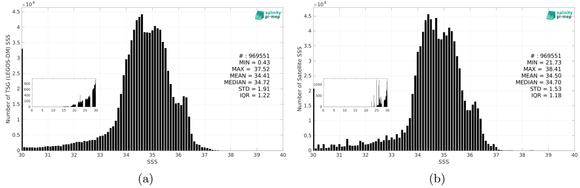
Figure 2: Histograms of SSS from TSG (LEGOS-DM) (a) and SMOS SSS L3 v9 - 18 Days (CATDS-CEC-LOCEAN) (b) considering all match-up pairs per bins of 0.1 over the Equatorial Ocean 10N-10S Pi-MEP region and for the full satellite product period.
