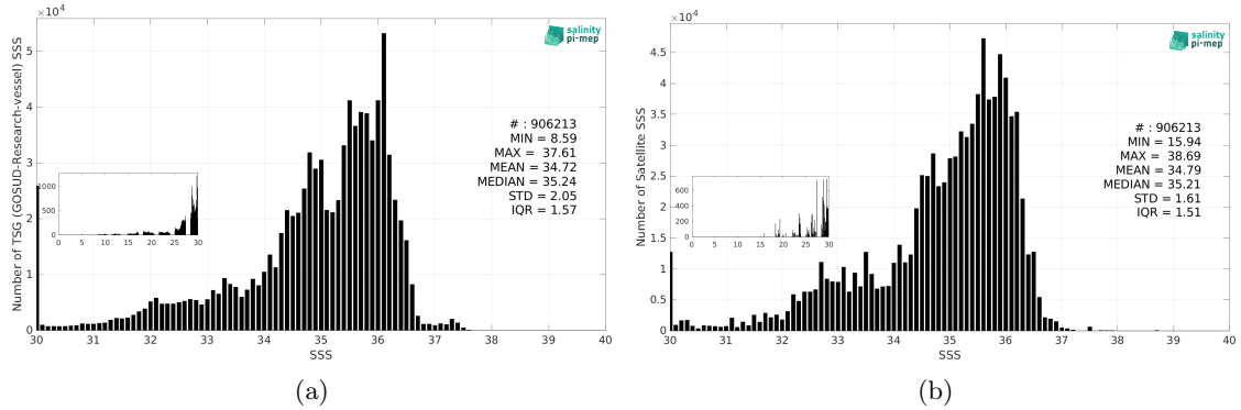
Figure 3: Histograms of SSS from TSG (GOSUD-Research-vessel) (a) and SMOS SSS L3 v9 - 18 Days (CATDS-CEC-LOCEAN) (b) considering all match-up pairs per bins of 0.1 over the Equatorial Ocean 10N-10S Pi-MEP region and for the full satellite product period.
