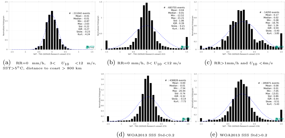
Figure 15: Normalized histogram of \Delta SSS (SMOS SSS L3 v9 - 18 Days (CATDS-CEC-LOCEAN) - TSG (GOSUD-Research-vessel)) for 5 different subdatasets corresponding to: RR=0 mm/h, 3 < U_{10} < 12 m/s, SST>5°C, distance to coast > 800 km (a), RR=0 mm/h, 3 < U_{10} < 12 m/s (b), RR>1mm/h and U_{10} < 4 m/s (c), WOA2013 SSS Std<0.2 (d), WOA2013 SSS Std>0.2 (e).
