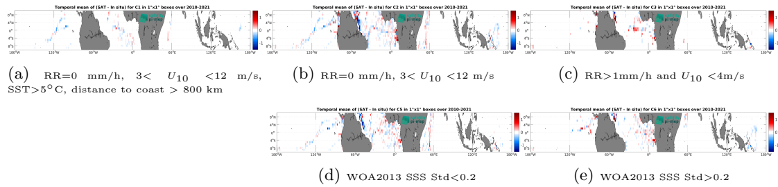
Figure 12: Temporal mean gridded over spatial boxes of size 1^\circ \times 1^\circ of \Delta SSS (SMOS SSS L3 v9 - 18 Days (CATDS-CEC-LOCEAN) - TSG (GOSUD-Research-vessel)) for 5 different subdatasets corresponding to:RR=0 mm/h, 3 < U_{10} < 12 m/s, SST>5°C, distance to coast > 800 km (a), RR=0 mm/h, 3 < U_{10} < 12 m/s (b), RR>1mm/h and U_{10} < 4 m/s (c), WOA2013 SSS Std<0.2 (d), WOA2013 SSS Std>0.2 (e).
