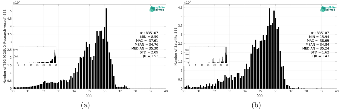
Figure 2: Histograms of SSS from TSG (GOSUD-Research-vessel) (a) and SMOS SSS L3 v9 - 18 Days (CATDS-CEC-LOCEAN) (b) considering all match-up pairs per bins of 0.1 over the Equatorial Ocean 10N-10S Pi-MEP region and for the full satellite product period.
