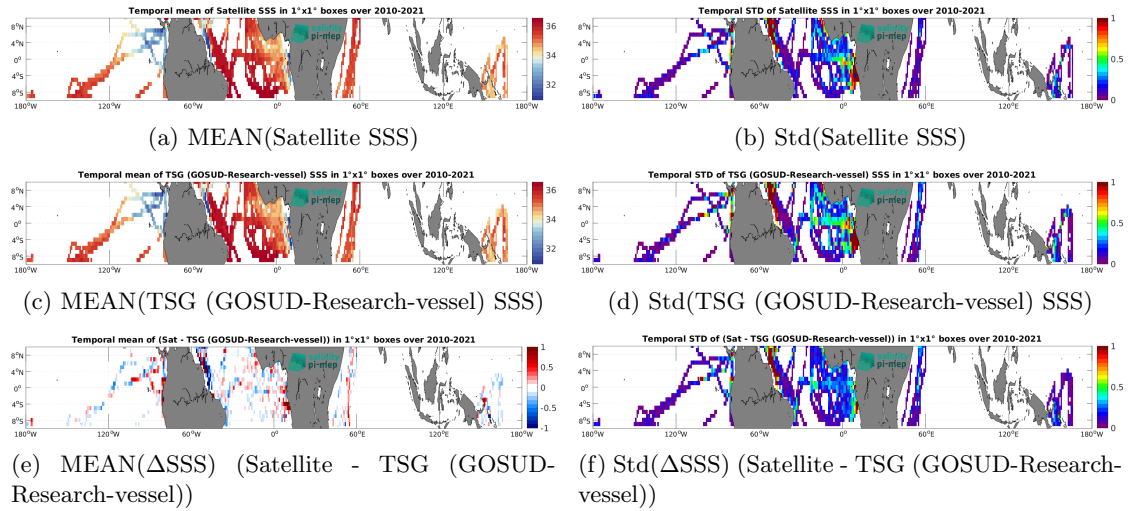
Figure 6: Temporal mean (left) and Std (right) of SSS from SMOS SSS L3 v9 - 18 Days (CATDS-CEC-LOCEAN) (top), TSG (GOSUD-Research-vessel) (middle), and of \Delta SSS (Satellite - TSG (GOSUD-Research-vessel)). Only match-up pairs are used to generate these maps.
