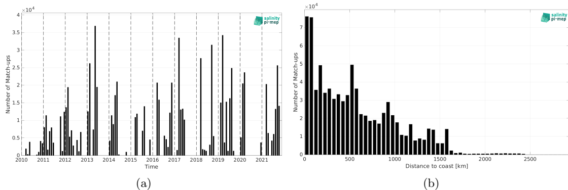
Figure 1: Number of match-ups between TSG (GOSUD-Research-vessel) and SMOS SSS L3 v9 - 18 Days (CATDS-CEC-LOCEAN) SSS as a function of time (a) and as function of the distance to coast (b) over the Equatorial Ocean 10N-10S Pi-MEP region and for the full satellite product period.
