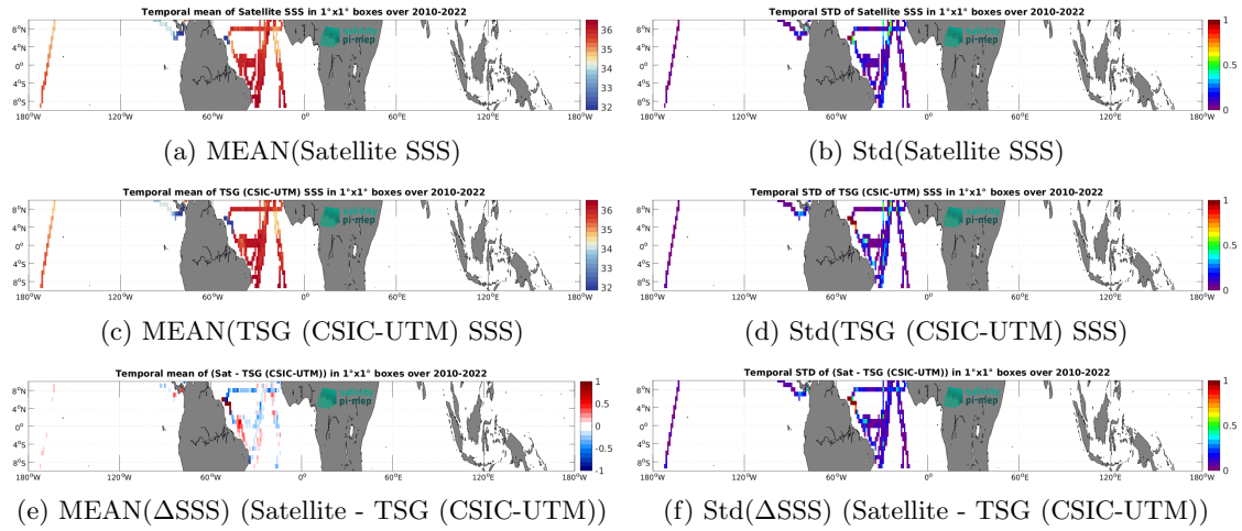
Figure 6: Temporal mean (left) and Std (right) of SSS from SMOS SSS L3 v9 - 18 Days (CATDS-CEC-LOCEAN) (top), TSG (CSIC-UTM) (middle), and of \Delta SSS (Satellite - TSG (CSIC-UTM)). Only match-up pairs are used to generate these maps.
