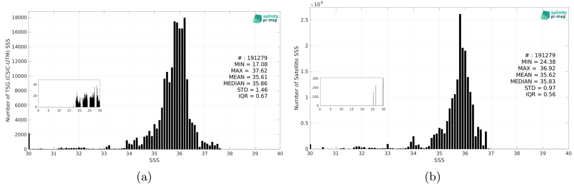
Figure 2: Histograms of SSS from TSG (CSIC-UTM) (a) and SMOS SSS L3 v9 - 18 Days (CATDS-CEC-LOCEAN) (b) considering all match-up pairs per bins of 0.1 over the Equatorial Ocean 10N-10S Pi-MEP region and for the full satellite product period.
