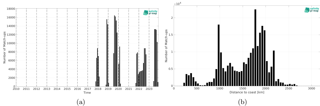
Figure 2: Number of match-ups between Saildrone and SMOS SSS L3 v9 - 18 Days (CATDS-CEC-LOCEAN) SSS as a function of time (a) and as function of the distance to coast (b) over the Equatorial Ocean 10N-10S Pi-MEP region and for the full satellite product period.
