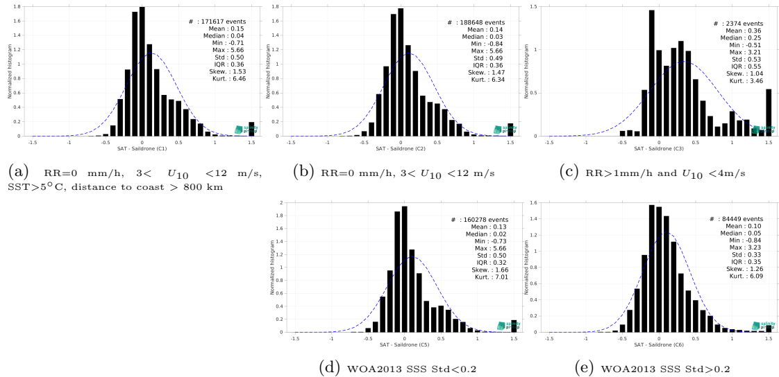
Figure 15: Normalized histogram of \Delta SSS (SMOS SSS L3 v9 - 18 Days (CATDS-CEC-LOCEAN) - Sailsdrone) for 5 different subdatasets corresponding to: RR=0 mm/h, 3 < U_{10} < 12 m/s, SST>5°C, distance to coast > 800 km (a), RR=0 mm/h, 3 < U_{10} < 12 m/s (b), RR>1mm/h and U_{10} < 4 m/s (c), WOA2013 SSS Std<0.2 (d), WOA2013 SSS Std>0.2 (e).
