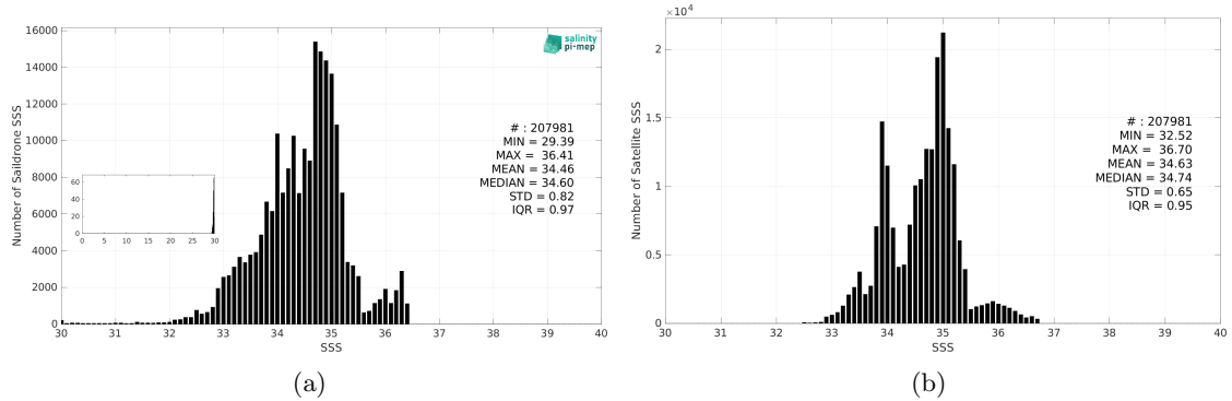
Figure 3: Histograms of SSS from Saildrone (a) and SMOS SSS L3 v9 - 18 Days (CATDS-CEC-LOCEAN) (b) considering all match-up pairs per bins of 0.1 over the Equatorial Ocean 10N-10S Pi-MEP region and for the full satellite product period.
