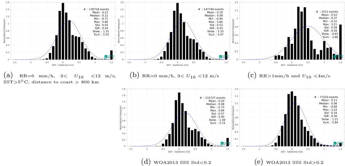
Figure 15: Normalized histogram of \Delta SSS (SMOS SSS L3 v9 - 18 Days (CATDS-CEC-LOCEAN) - Sailydrone) for 5 different subdatasets corresponding to: RR=0 mm/h, 3 < U_{10} < 12 m/s, SST>5°C, distance to coast > 800 km (a), RR=0 mm/h, 3 < U_{10} < 12 m/s (b), RR>1mm/h and U_{10} < 4 m/s (c), WOA2013 SSS Std<0.2 (d), WOA2013 SSS Std>0.2 (e).
