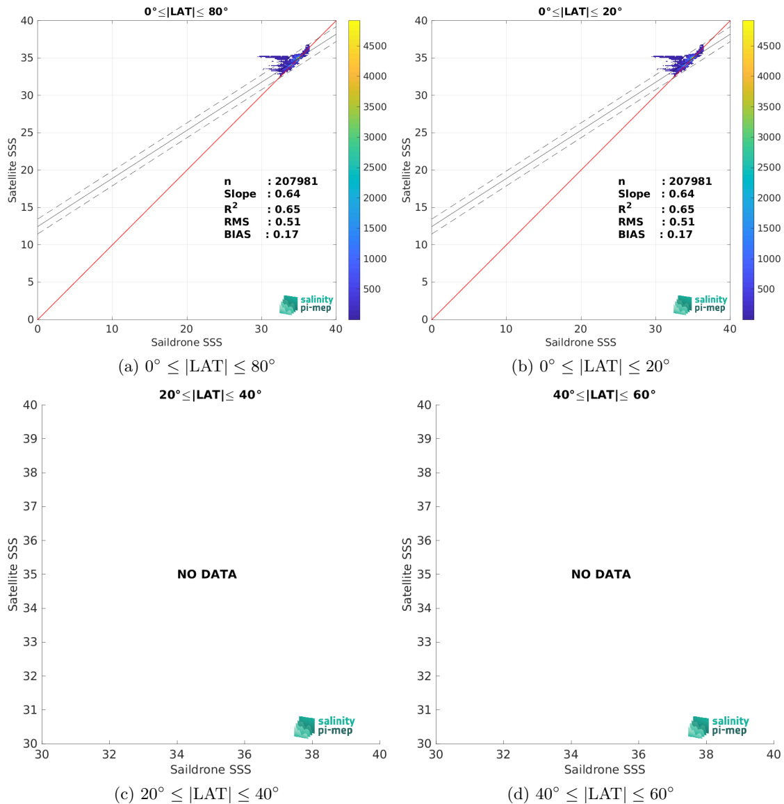
Figure 10: Contour maps of the concentration of SMOS SSS L3 v9 - 18 Days (CATDS-CEC-LOCEAN) SSS (y-axis) versus Saildrone SSS (x-axis) at match-up pairs for different latitude bands. For each plot, the red line shows x=y . The black thin and dashed lines indicate a linear fit through the data cloud and the \pm 95\% confidence levels, respectively. The number match-up pairs n , the slope and R^2 coefficient of the linear fit, the root mean square (RMS) and the mean bias between satellite and in situ data are indicated for each latitude band in each plots.
