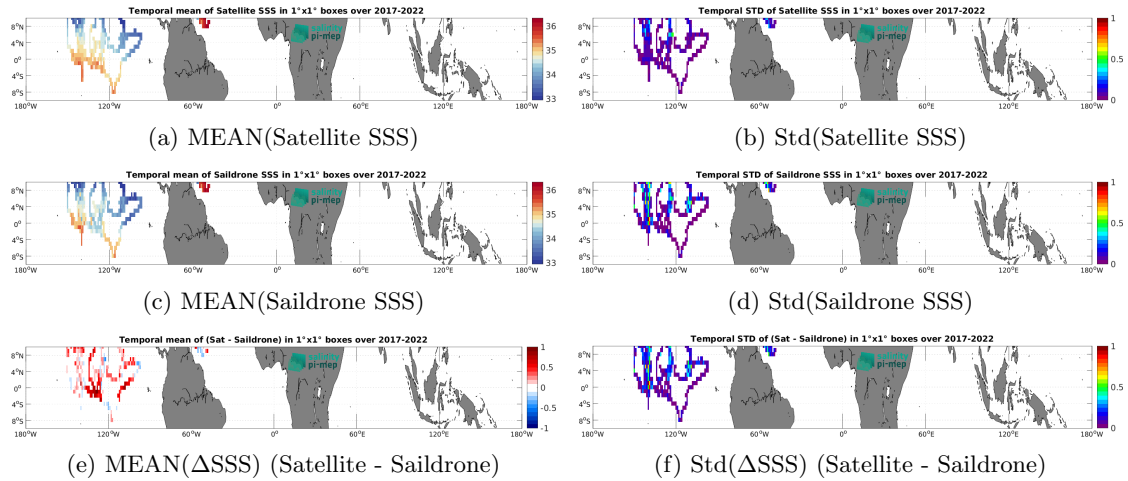
Figure 7: Temporal mean (left) and Std (right) of SSS from SMOS SSS L3 v9 - 18 Days (CATDS-CEC-LOCEAN) (top), Saildrone (middle), and of \Delta SSS (Satellite - Saildrone). Only match-up pairs are used to generate these maps.
