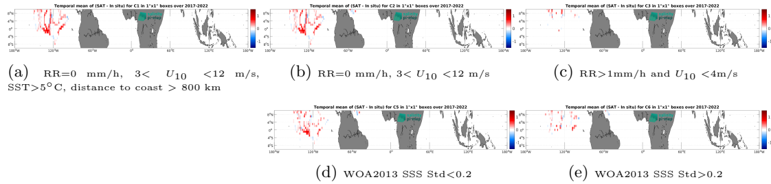
Figure 14: Temporal mean gridded over spatial boxes of size 1^\circ \times 1^\circ of \Delta SSS (SMOS SSS L3 v9 - 18 Days (CATDS-CEC-LOCEAN) - Sailydrone) for 5 different subdatasets corresponding to: RR=0 mm/h, 3 < U_{10} < 12 m/s, SST>5°C, distance to coast > 800 km (a), RR=0 mm/h, 3 < U_{10} < 12 m/s (b), RR>1mm/h and U_{10} < 4 m/s (c), WOA2013 SSS Std<0.2 (d), WOA2013 SSS Std>0.2 (e).
