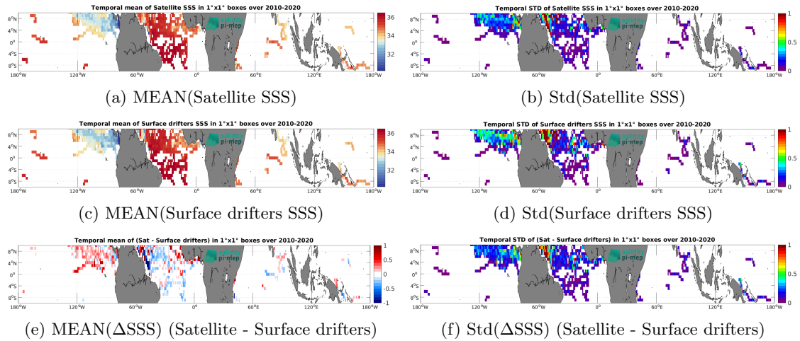
Figure 5: Temporal mean (left) and Std (right) of SSS from SMOS SSS L3 v9 - 18 Days (CATDS-CEC-LOCEAN) (top), Surface drifters (middle), and of \Delta SSS (Satellite - Surface drifters). Only match-up pairs are used to generate these maps.
