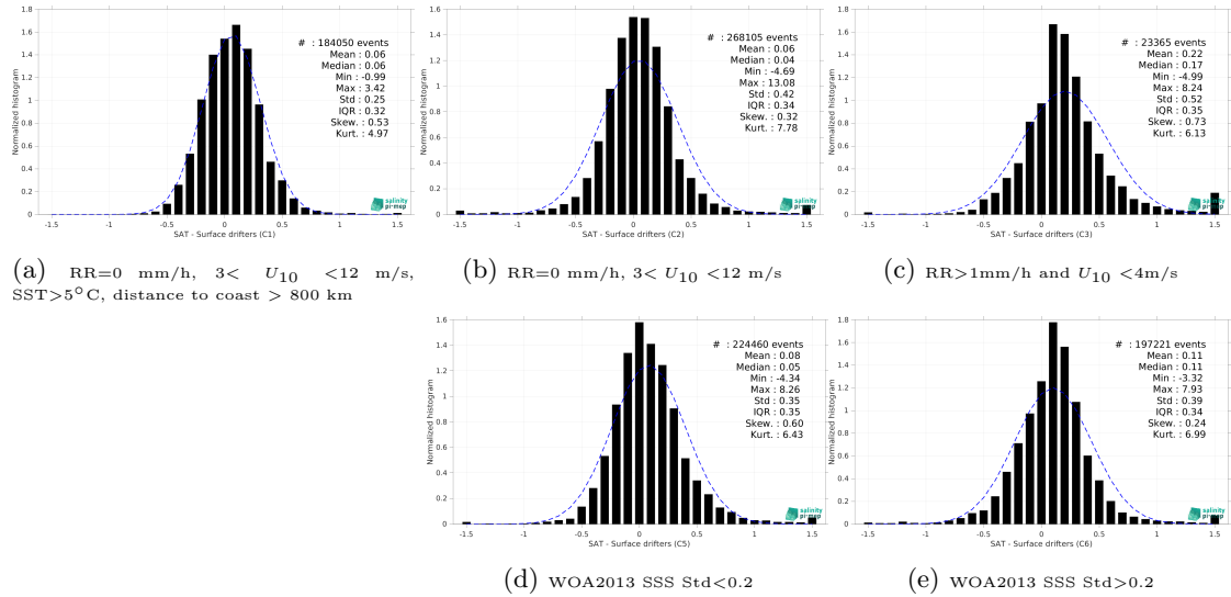
Figure 12: Normalized histogram of \Delta SSS (SMOS SSS L3 v9 - 18 Days (CATDS-CEC-LOCEAN) - Surface drifters) for 5 different subdatasets corresponding to: RR=0 mm/h, 3 < U_{10} < 12 m/s, SST >5^\circ\text{C} , distance to coast > 800 km (a), RR=0 mm/h, 3 < U_{10} < 12 m/s (b), RR >1 mm/h and U_{10} < 4 m/s (c), WOA2013 SSS Std <0.2 (d), WOA2013 SSS Std >0.2 (e).
