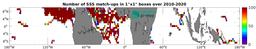
Figure 3: Number of SSS match-ups between Surface drifters SSS and the SMOS SSS L3 v9 - 18 Days (CATDS-CEC-LOCEAN) SSS product for the Equatorial Ocean 10N-10S Pi-MEP region over 1^\circ \times 1^\circ boxes and for the full satellite product period.
