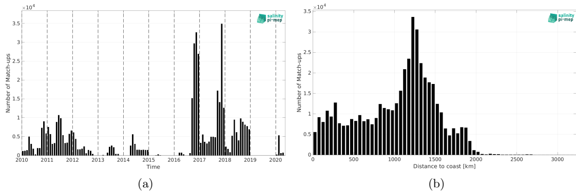
Figure 1: Number of match-ups between Surface drifters and SMOS SSS L3 v9 - 18 Days (CATDS-CEC-LOCEAN) SSS as a function of time (a) and as function of the distance to coast (b) over the Equatorial Ocean 10N-10S Pi-MEP region and for the full satellite product period.
