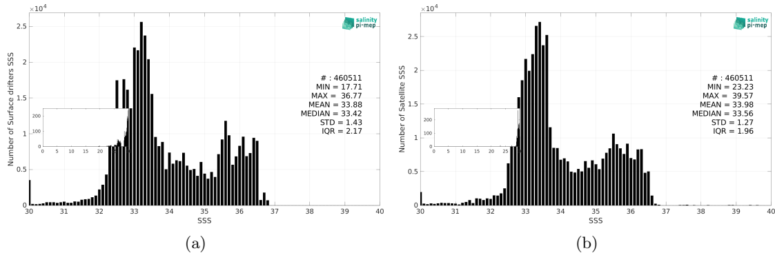
Figure 2: Histograms of SSS from Surface drifters (a) and SMOS SSS L3 v9 - 18 Days (CATDS-CEC-LOCEAN) (b) considering all match-up pairs per bins of 0.1 over the Equatorial Ocean 10N-10S Pi-MEP region and for the full satellite product period.
