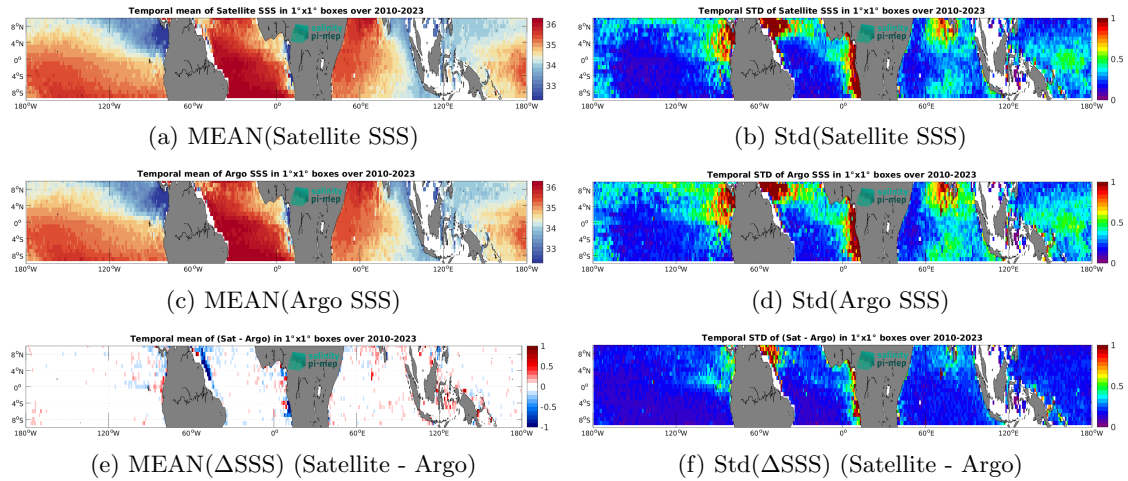
Figure 6: Temporal mean (left) and Std (right) of SSS from SMOS SSS L3 v9 - 18 Days (CATDS-CEC-LOCEAN) (top), Argo (middle), and of \Delta SSS (Satellite - Argo). Only match-up pairs are used to generate these maps.
