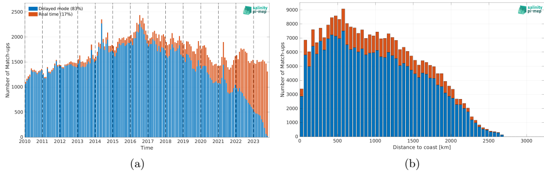
Figure 1: Number of match-ups between Argo and SMOS SSS L3 v9 - 18 Days (CATDS-CEC-LOCEAN) SSS as a function of time (a) and as function of the distance to coast (b) over the Equatorial Ocean 10N-10S Pi-MEP region and for the full satellite product period.
