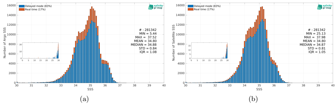
Figure 2: Histograms of SSS from Argo (a) and SMOS SSS L3 v9 - 18 Days (CATDS-CEC-LOCEAN) (b) considering all match-up pairs per bins of 0.1 over the Equatorial Ocean 10N-10S Pi-MEP region and for the full satellite product period.
