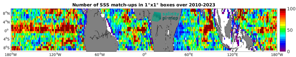
Figure 4: Number of SSS match-ups between Argo SSS and the SMOS SSS L3 v9 - 18 Days (CATDS-CEC-LOCEAN) SSS product for the Equatorial Ocean 10N-10S Pi-MEP region over 1^\circ \times 1^\circ boxes and for the full satellite product period.
