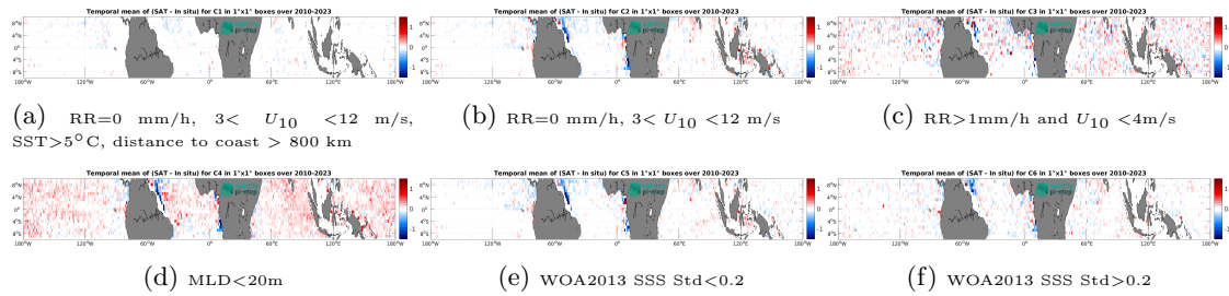
Figure 12: Temporal mean gridded over spatial boxes of size 1^\circ \times 1^\circ of \Delta SSS (SMOS SSS L3 v9 - 18 Days (CATDS-CEC-LOCEAN) - Argo) for 6 different subdatasets corresponding to:RR=0 mm/h, 3 < U_{10} < 12 m/s, SST >5^\circ C, distance to coast > 800 km (a), RR=0 mm/h, 3 < U_{10} < 12 m/s (b), RR >1 mm/h and U_{10} < 4 m/s (c),MLD <20 m (d),WOA2013 SSS Std <0.2 (e),WOA2013 SSS Std >0.2 (f).
