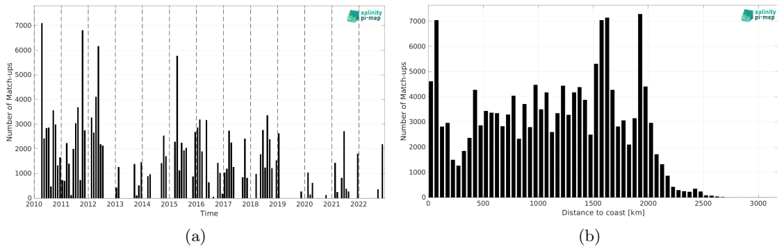
Figure 1: Number of match-ups between TSG (SAMOS) and SMOS SSS L3 v8 - 9 Days (CATDS-CEC-LOCEAN) SSS as a function of time (a) and as function of the distance to coast (b) over the Equatorial Ocean 10N-10S Pi-MEP region and for the full satellite product period.
