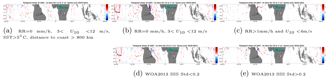
Figure 12: Temporal mean gridded over spatial boxes of size 1^\circ \times 1^\circ of \Delta SSS (SMOS SSS L3 v8 - 9 Days (CATDS-CEC-LOCEAN) - TSG (SAMOS)) for 5 different subdatasets corresponding to:RR=0 mm/h, 3 < U_{10} < 12 m/s, SST >5^\circ C, distance to coast > 800 km (a), RR=0 mm/h, 3 < U_{10} < 12 m/s (b), RR >1 mm/h and U_{10} < 4 m/s (c), WOA2013 SSS Std <0.2 (d), WOA2013 SSS Std >0.2 (e).
