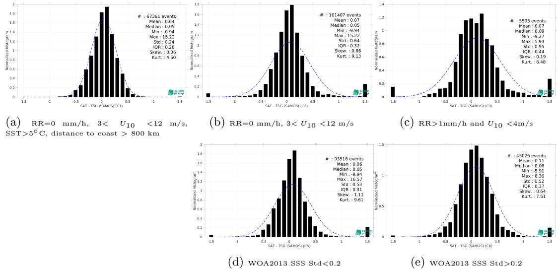
Figure 13: Normalized histogram of \Delta SSS (SMOS SSS L3 v8 - 9 Days (CATDS-CEC-LOCEAN) - TSG (SAMOS)) for 5 different subdatasets corresponding to: RR=0 mm/h, 3 < U_{10} < 12 m/s, SST >5^\circ C, distance to coast > 800 km (a), RR=0 mm/h, 3 < U_{10} < 12 m/s (b), RR >1 mm/h and U_{10} < 4 m/s (c), WOA2013 SSS Std <0.2 (d), WOA2013 SSS Std >0.2 (e).
