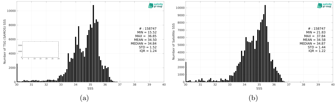
Figure 2: Histograms of SSS from TSG (SAMOS) (a) and SMOS SSS L3 v8 - 9 Days (CATDS-CEC-LOCEAN) (b) considering all match-up pairs per bins of 0.1 over the Equatorial Ocean 10N-10S Pi-MEP region and for the full satellite product period.
