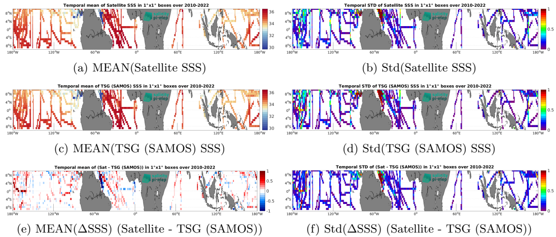
Figure 6: Temporal mean (left) and Std (right) of SSS from SMOS SSS L3 v8 - 9 Days (CATDS-CEC-LOCEAN) (top), TSG (SAMOS) (middle), and of \Delta SSS (Satellite - TSG (SAMOS)). Only match-up pairs are used to generate these maps.
