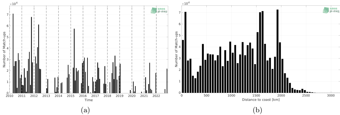
Figure 1: Number of match-ups between TSG (SAMOS) and SMOS SSS L3 v8 - 9 Days (CATDS-CECOS-LOCEAN) SSS as a function of time (a) and as function of the distance to coast (b) over the Equatorial Ocean 10N-10S Pi-MEP region and for the full satellite product period.
