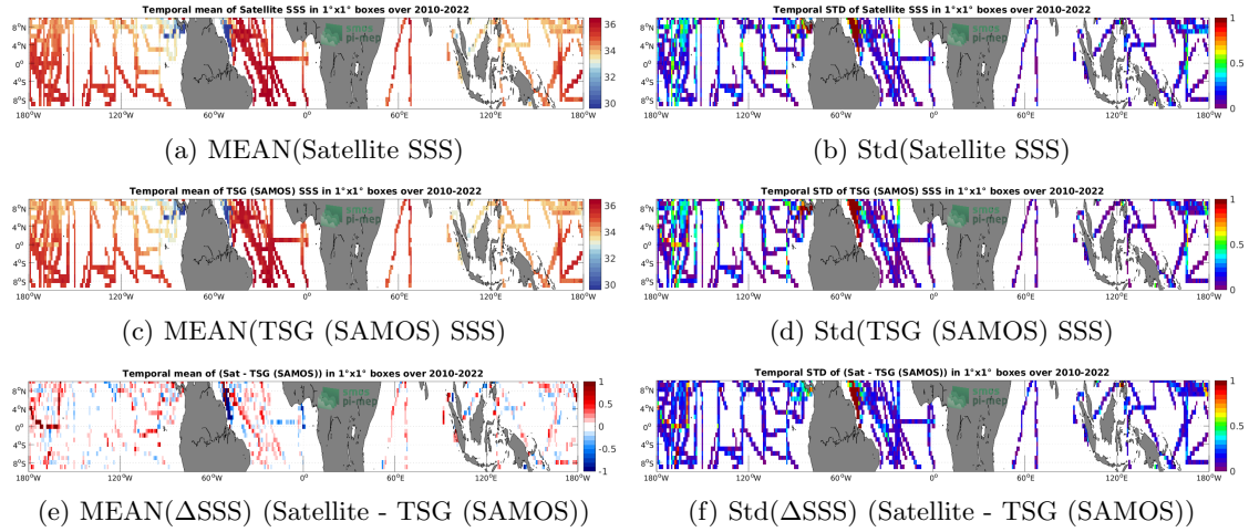
Figure 6: Temporal mean (left) and Std (right) of SSS from SMOS SSS L3 v8 - 9 Days (CATDS-CECOS-LOCEAN) (top), TSG (SAMOS) ( in situ ) (middle), and of \Delta SSS (Satellite - TSG (SAMOS)). Only match-up pairs are used to generate these maps.
