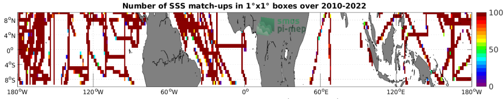
Figure 4: Number of SSS match-ups between TSG (SAMOS) SSS and the SMOS SSS L3 v8 - 9 Days (CATDS-CECOS-LOCEAN) SSS product for the Equatorial Ocean 10N-10S Pi-MEP region over 1^\circ \times 1^\circ boxes and for the full satellite product period.
