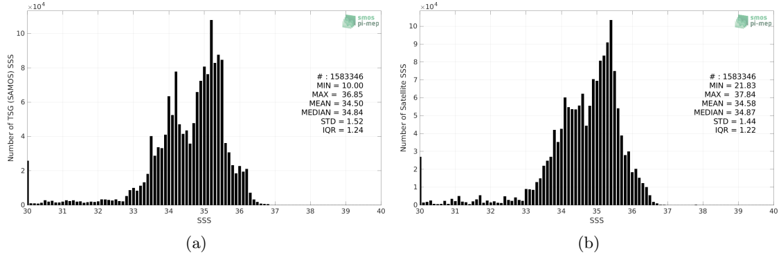
Figure 2: Histograms of SSS from TSG (SAMOS) (a) and SMOS SSS L3 v8 - 9 Days (CATDS-CECOS-LOCEAN) (b) considering all match-up pairs per bins of 0.1 over the Equatorial Ocean 10N-10S Pi-MEP region and for the full satellite product period.
