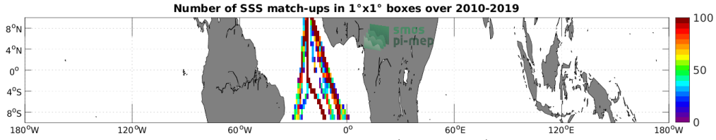
Figure 4: Number of SSS match-ups between TSG (Polarstern) SSS and the SMOS SSS L3 v8 - 9 Days (CATDS-CECOS-LOCEAN) SSS product for the Equatorial Ocean 10N-10S Pi-MEP region over 1^\circ \times 1^\circ boxes and for the full satellite product period.
