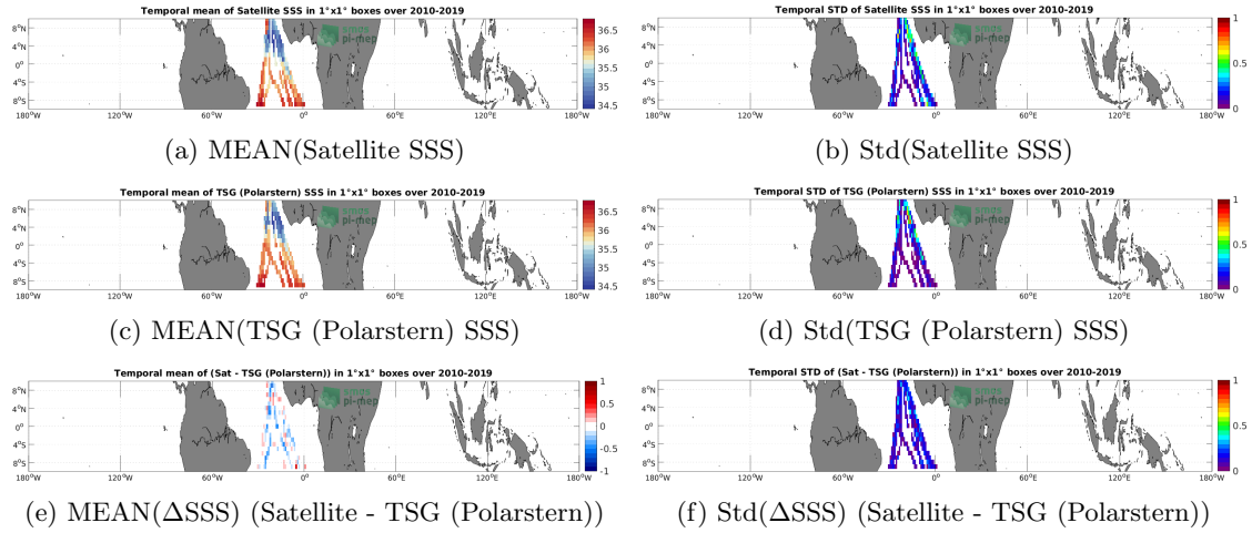
Figure 6: Temporal mean (left) and Std (right) of SSS from SMOS SSS L3 v8 - 9 Days (CATDS-CECOS-LOCEAN) (top), TSG (Polarstern) (middle), and of \Delta SSS (Satellite - TSG (Polarstern)). Only match-up pairs are used to generate these maps.
