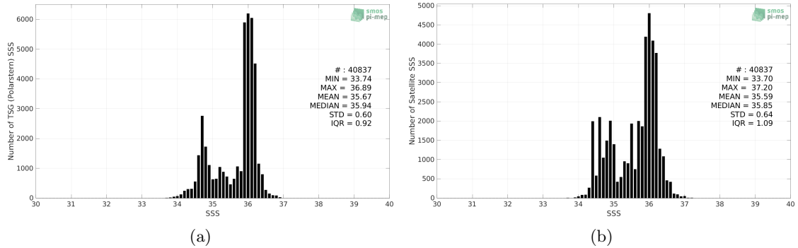
Figure 2: Histograms of SSS from TSG (Polarstern) (a) and SMOS SSS L3 v8 - 9 Days (CATDS-CECOS-LOCEAN) (b) considering all match-up pairs per bins of 0.1 over the Equatorial Ocean 10N-10S Pi-MEP region and for the full satellite product period.
