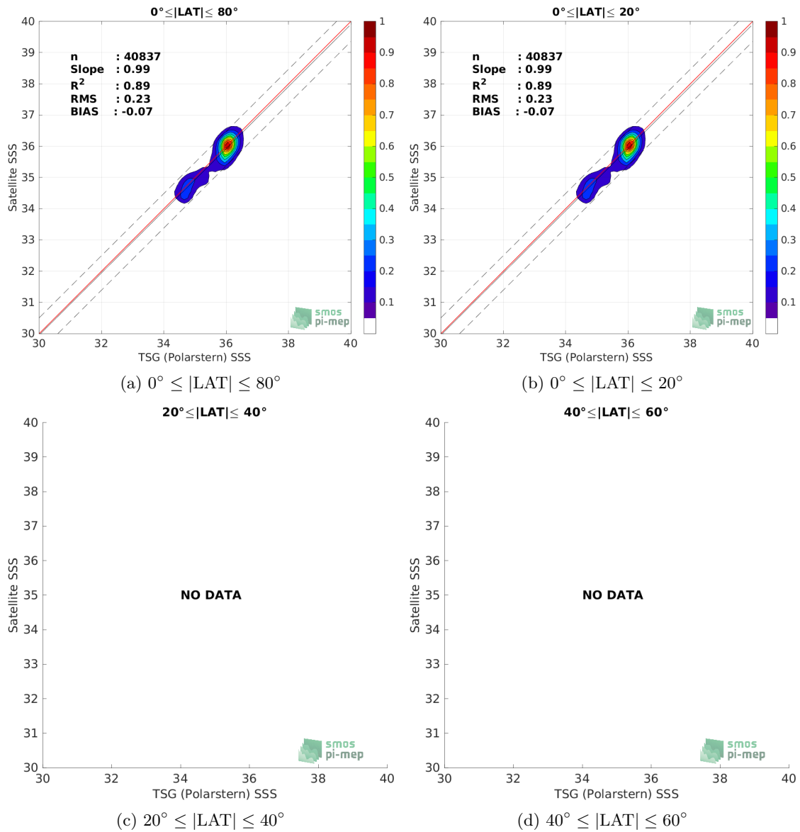
Figure 9: Contour maps of the concentration of SMOS SSS L3 v8 - 9 Days (CATDS-CECOS-LOCEAN) SSS (y-axis) versus TSG (Polarstern) SSS (x-axis) at match-up pairs for different latitude bands. For each plot, the red line shows x=y . The black thin and dashed lines indicate a linear fit through the data cloud and the \pm 95\% confidence levels, respectively. The number match-up pairs n , the slope and R^2 coefficient of the linear fit, the root mean square (RMS) and the mean bias between satellite and in situ data are indicated for each latitude band in each plots.
