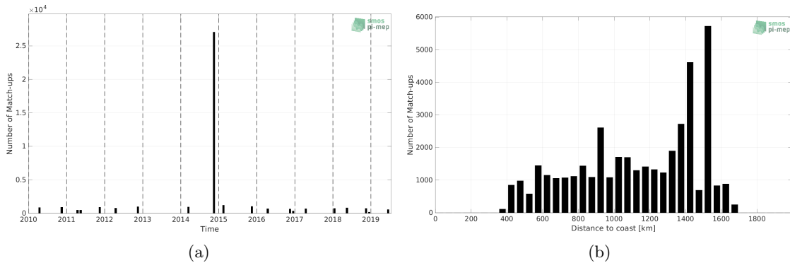
Figure 1: Number of match-ups between TSG (Polarstern) and SMOS SSS L3 v8 - 9 Days (CATDS-CECOS-LOCEAN) SSS as a function of time (a) and as function of the distance to coast (b) over the Equatorial Ocean 10N-10S Pi-MEP region and for the full satellite product period.
